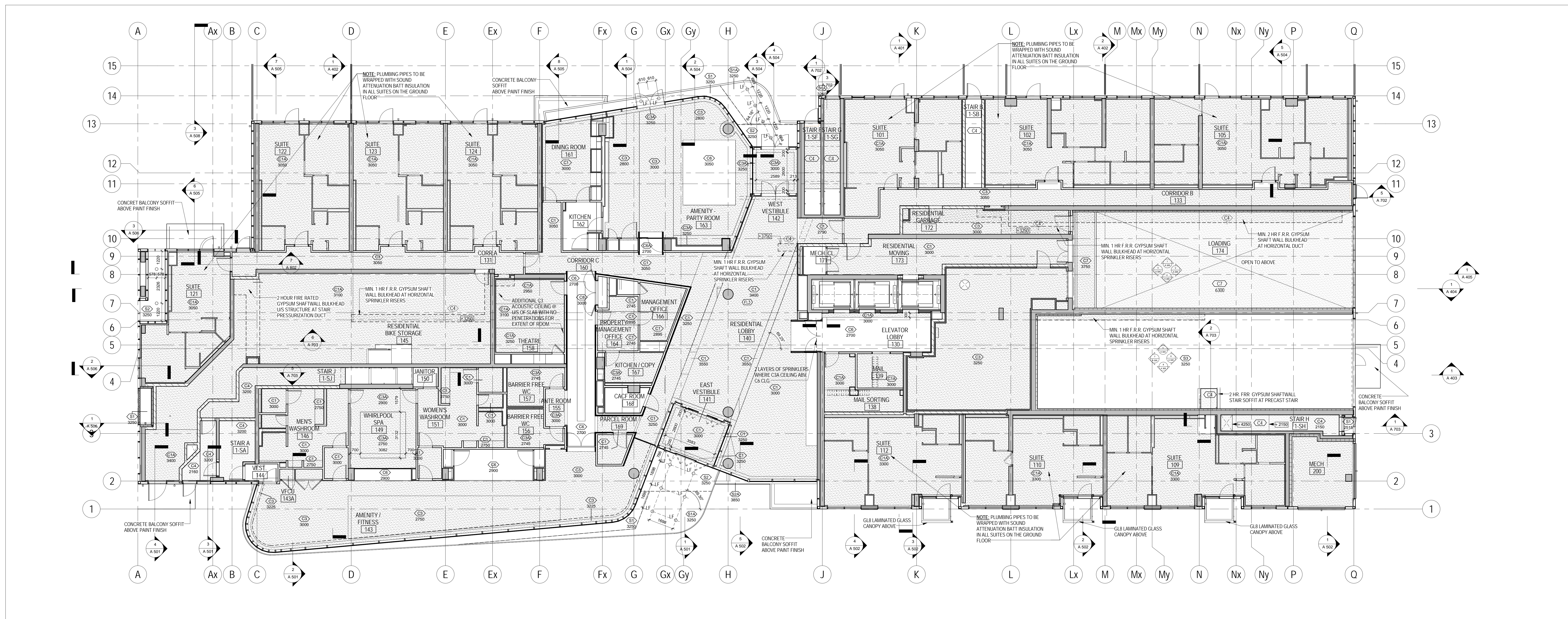
2 REFLECTED CEILING PLAN LEVEL 1 A 261 1:100
