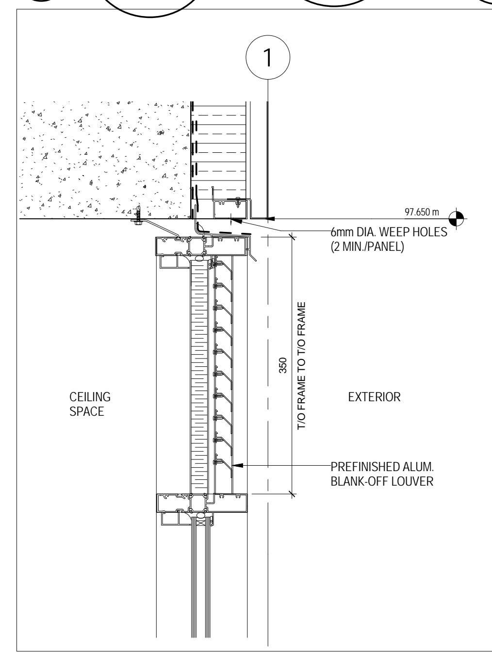
3B TYPICAL LOUVER DETAIL 1/4 (A 502) 1:5
