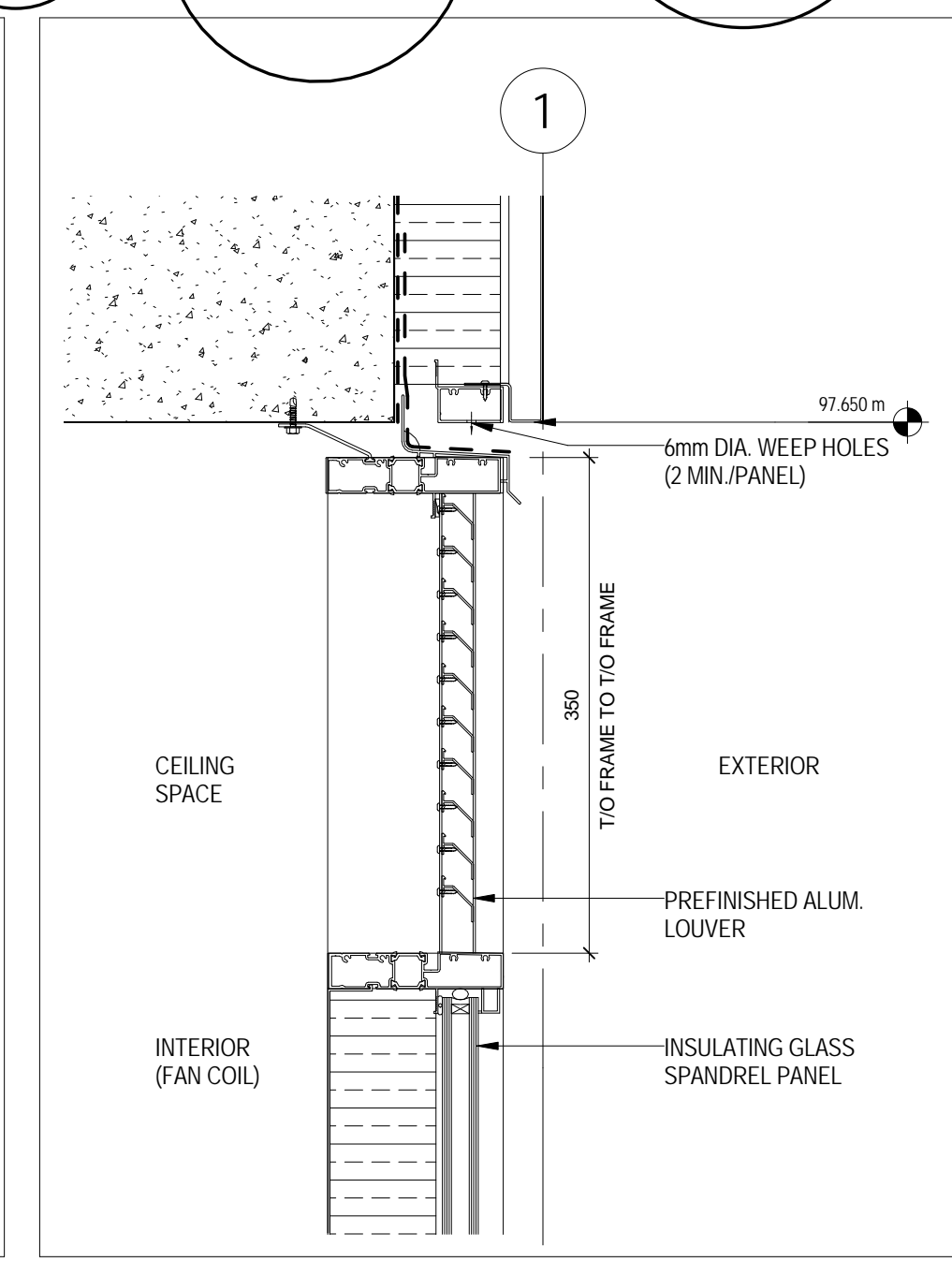
3A TYPICAL LOUVER DETAIL 1/4 (A 502) 1:5
