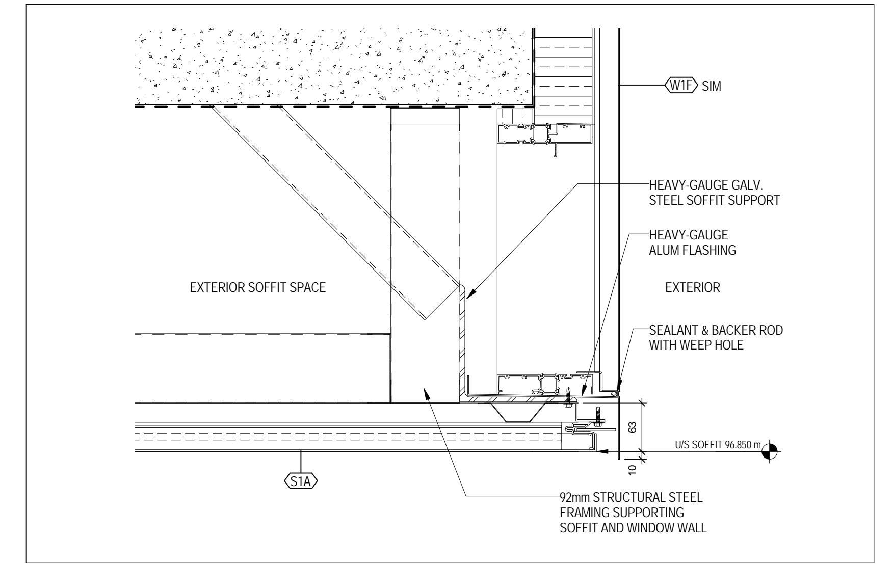
2A TYPICAL SOFFIT DETAIL 1/1 (A 501) 1:5
