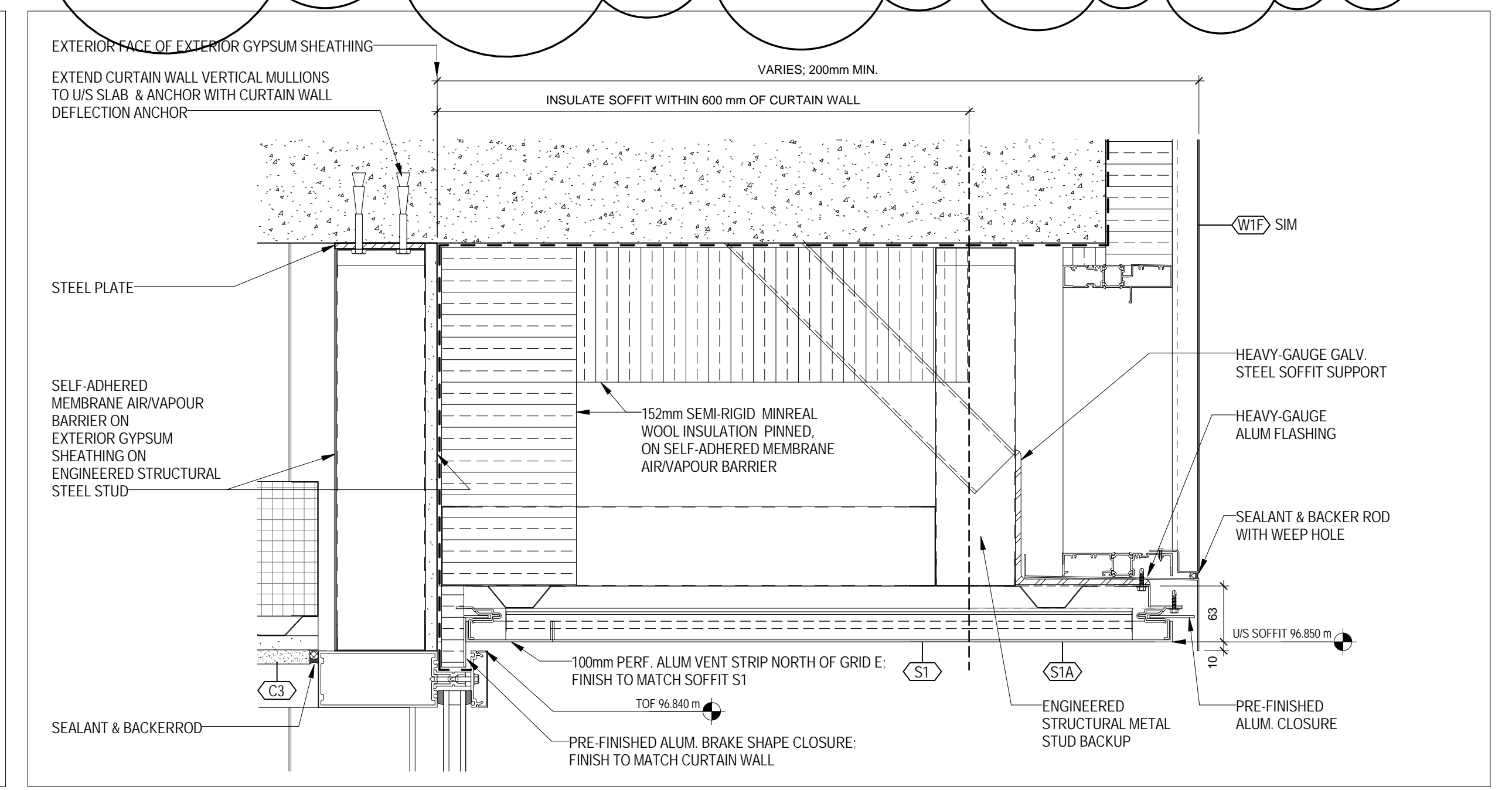
2 TYPICAL SOFFIT DETAIL 1/1 (A 252) 1:5
