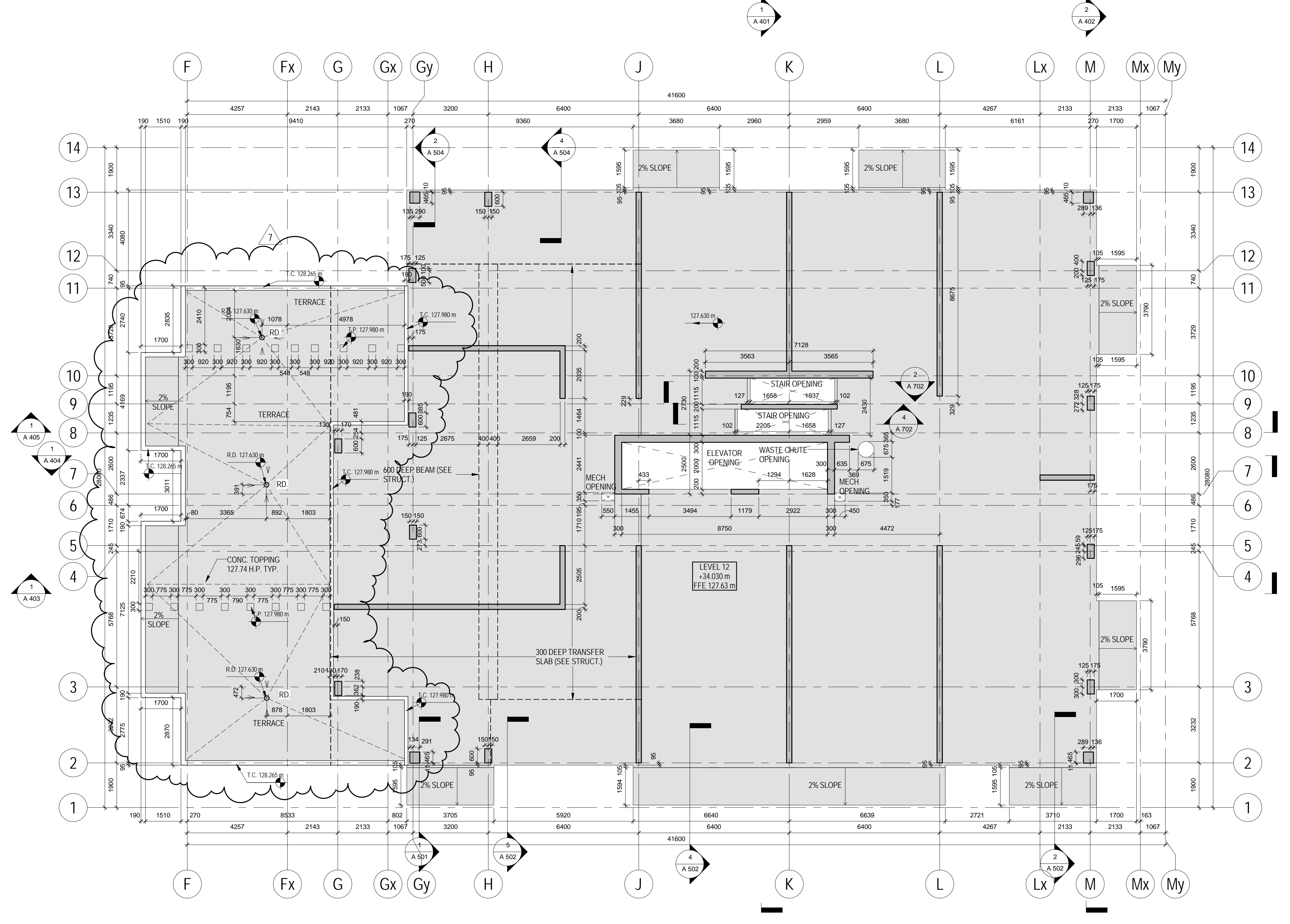
2 Level 12 EOS 1/A227 1:100
