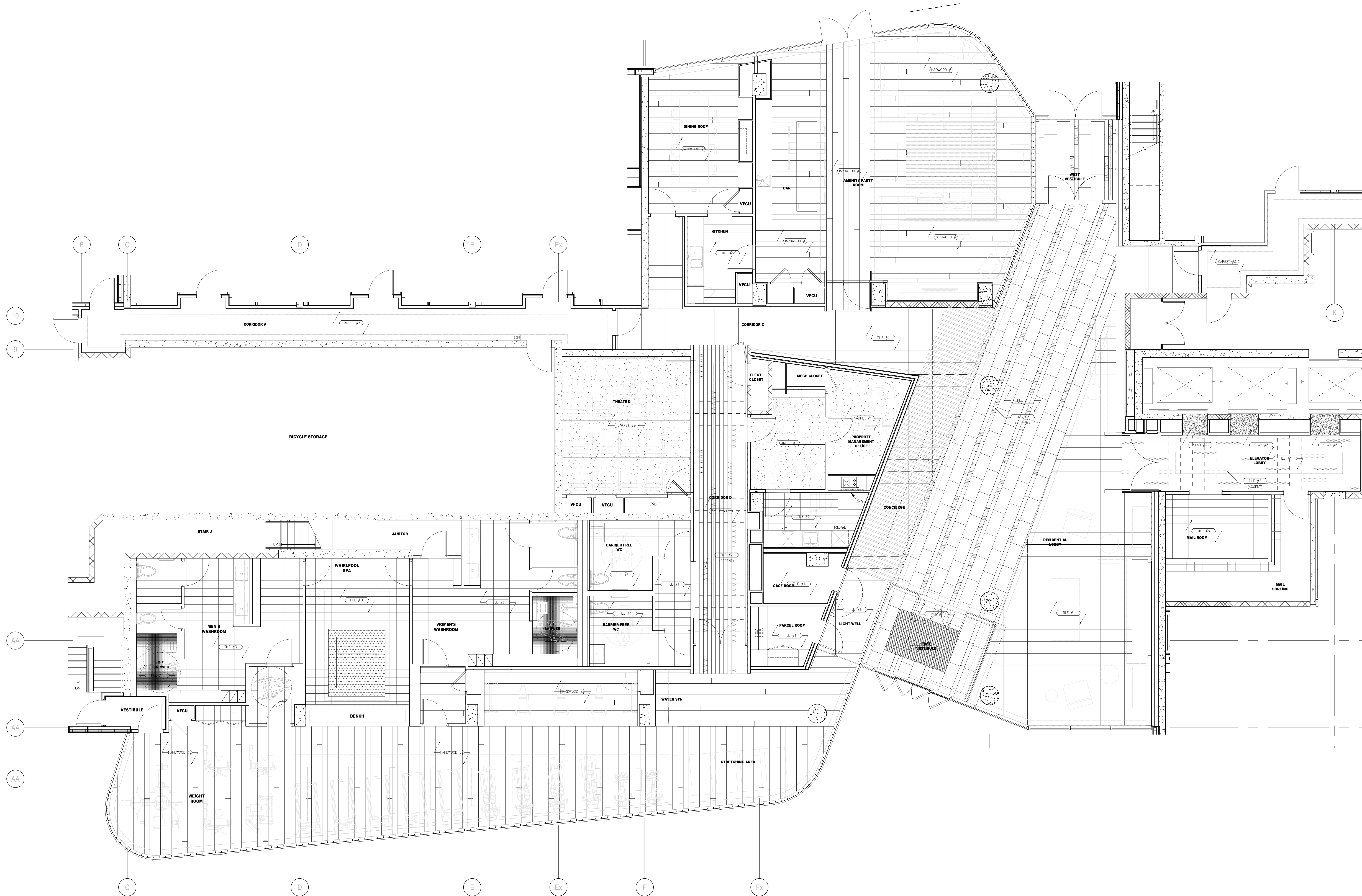
1 FLOOR FINISHES PLAN ID1.1.3 GROUND FLOOR SCALE 1:50
