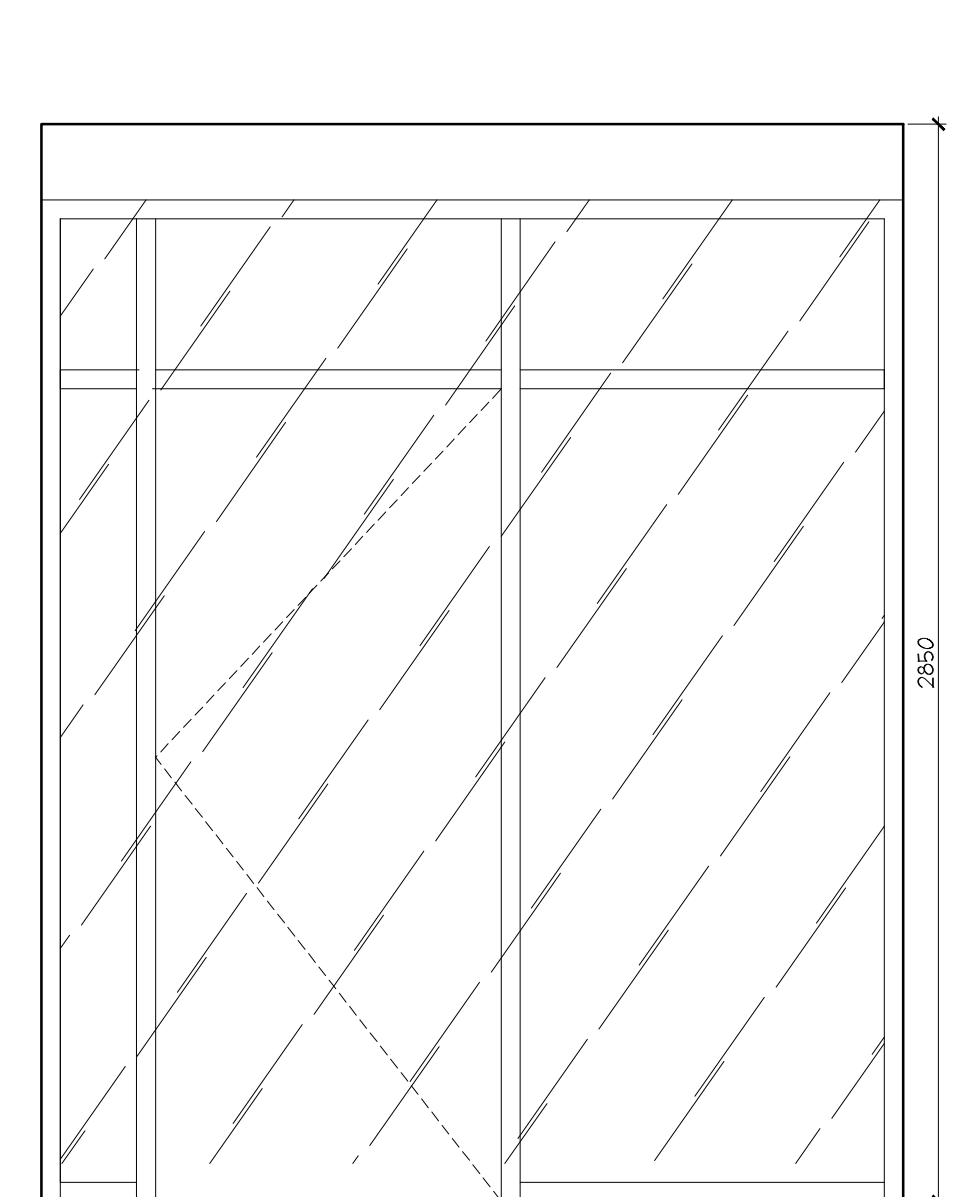
5 ELEVATION ID2.0.1 P1 LEVEL VESTIBULE SCALE 1:20
