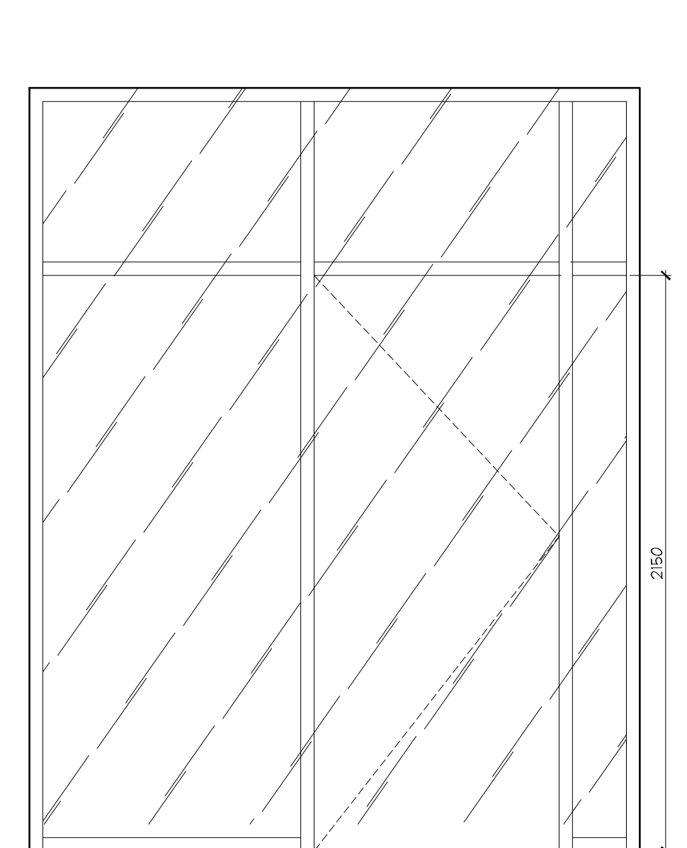
6 ELEVATION ID2.0.1 P1 LEVEL VESTIBULE SCALE 1:20
