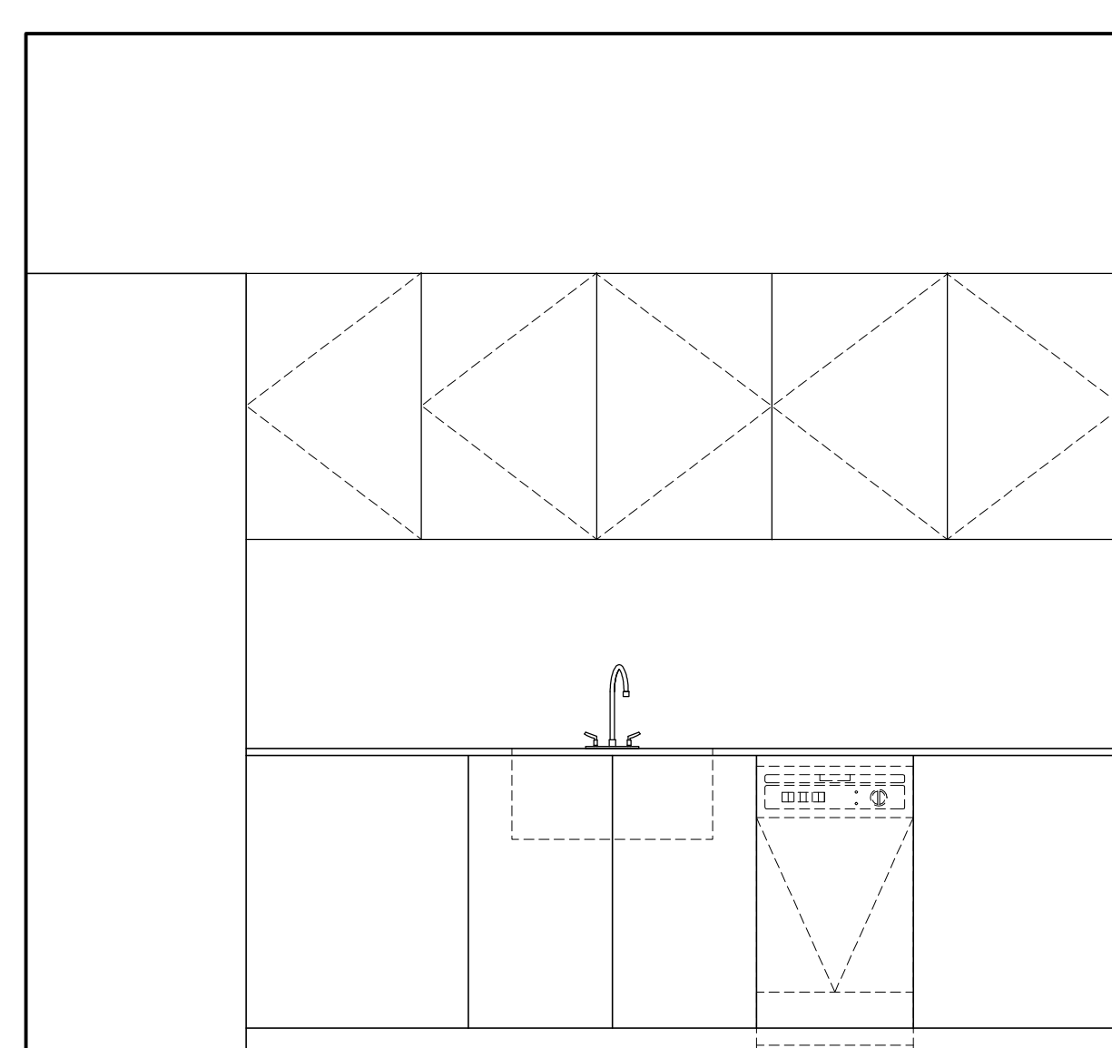
6 ELEVATION ID2.1.4 GROUND FLOOR KITCHEN SCALE 1:20
