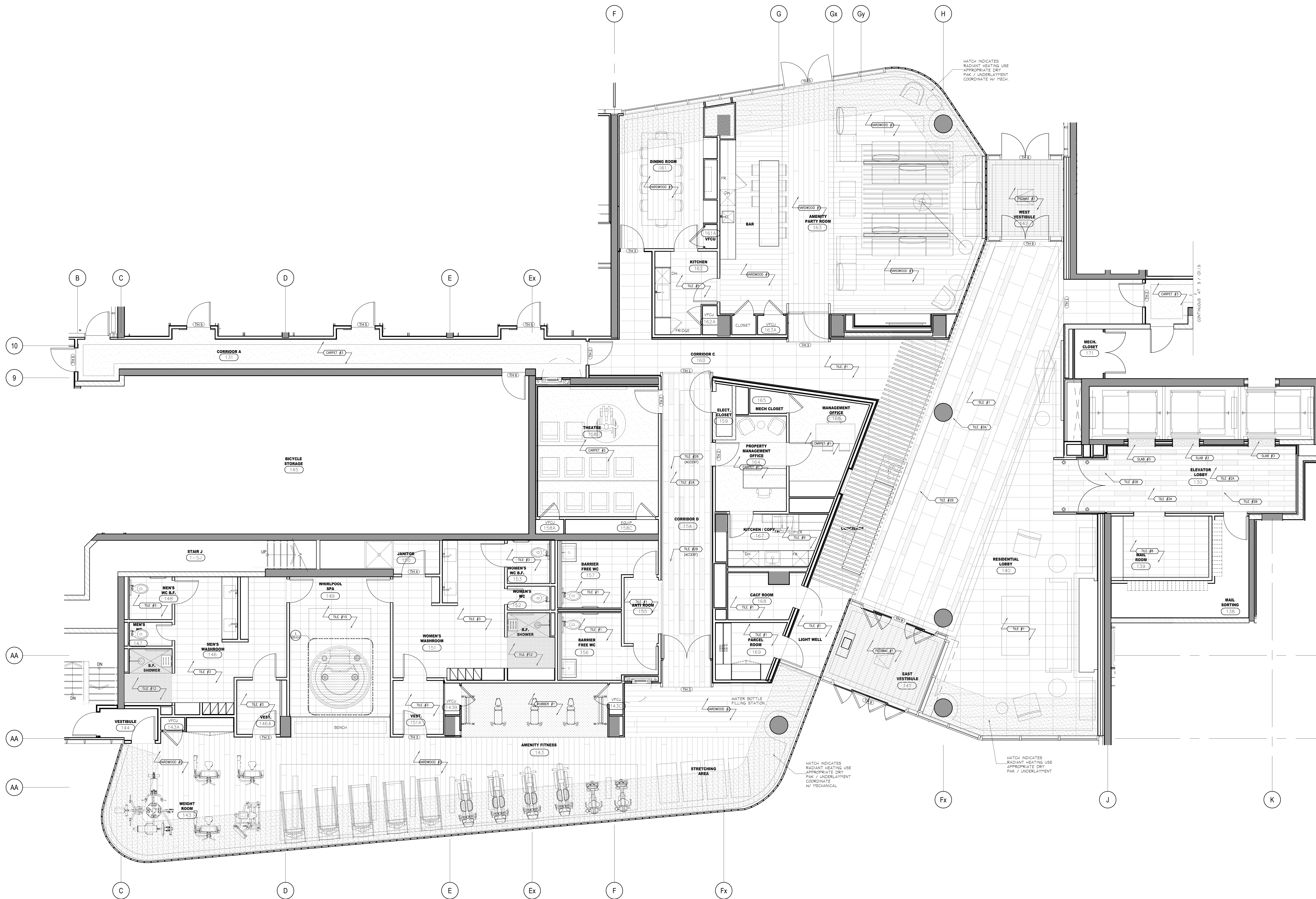
1 FLOOR FINISHES PLAN GROUND FLOOR SCALE: 1/8" = 1'-0"
