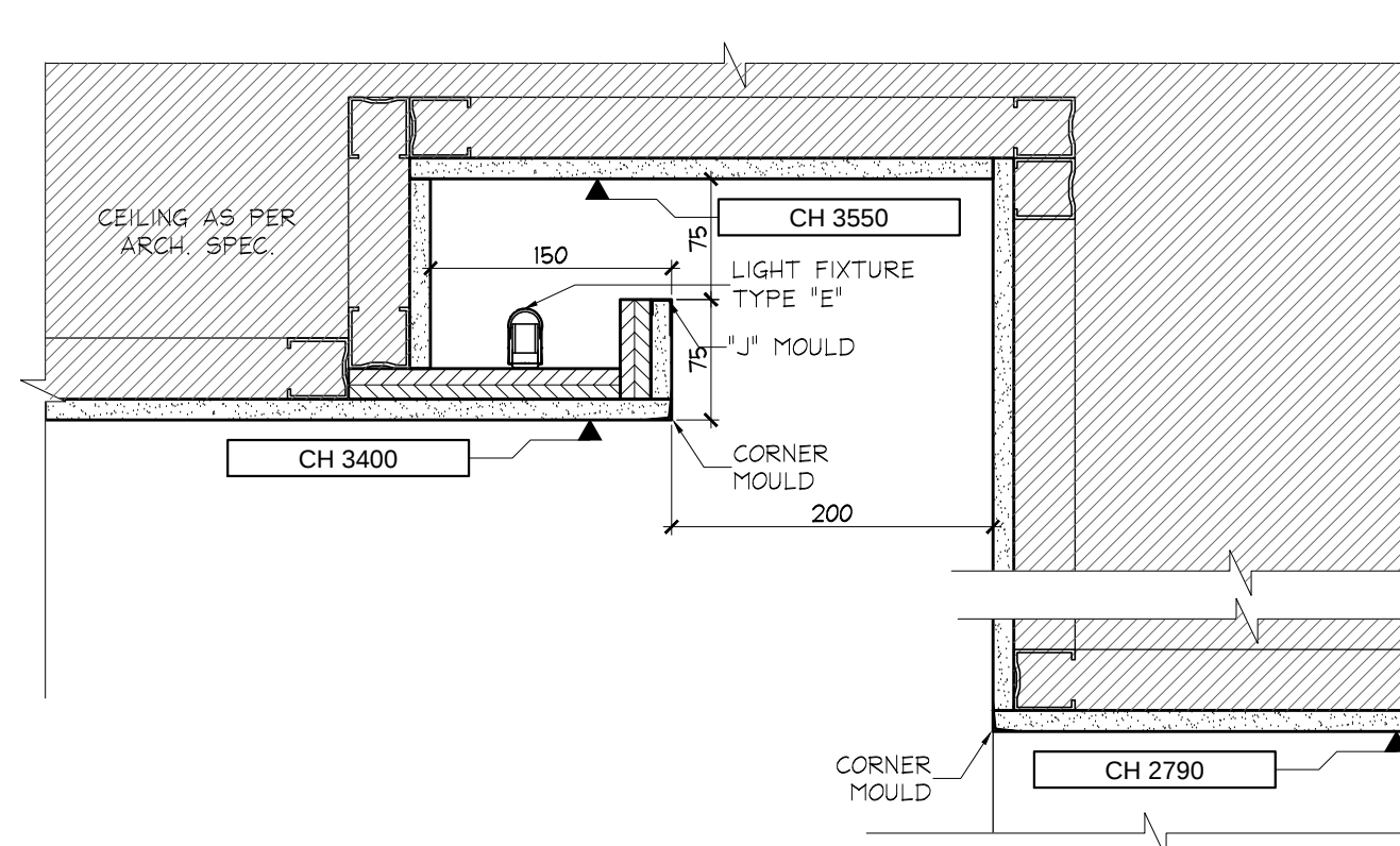
10 SECTION ID3.1.0 1ST FLOOR SCALE 1:5
