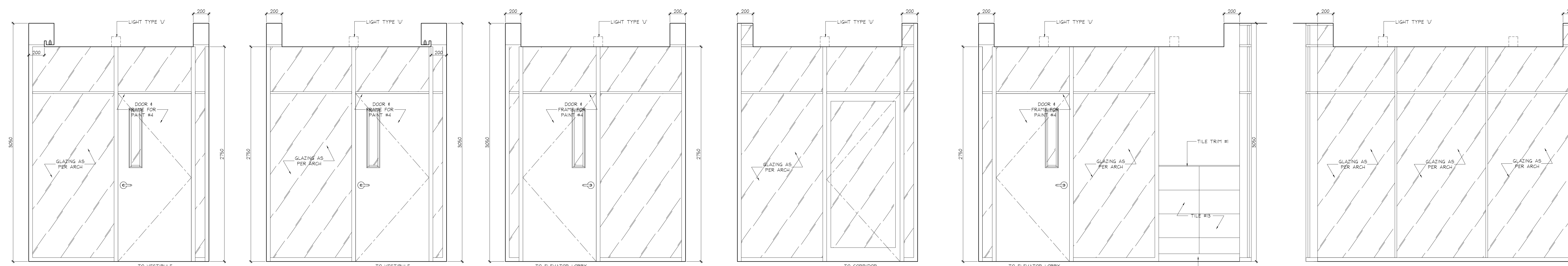
3 ELEVATION ID2.0.1 P1 LEVEL ELEVATOR LOBBY SCALE 1:20
