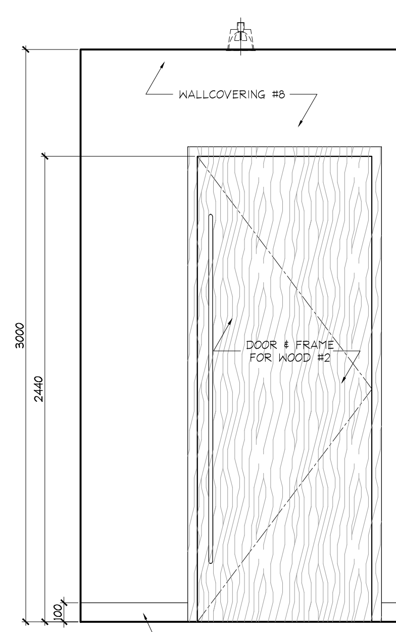
5 ELEVATION GROUND FLOOR WOMEN'S/MEN'S W.R. VESTIBULE SCALE 1:20
