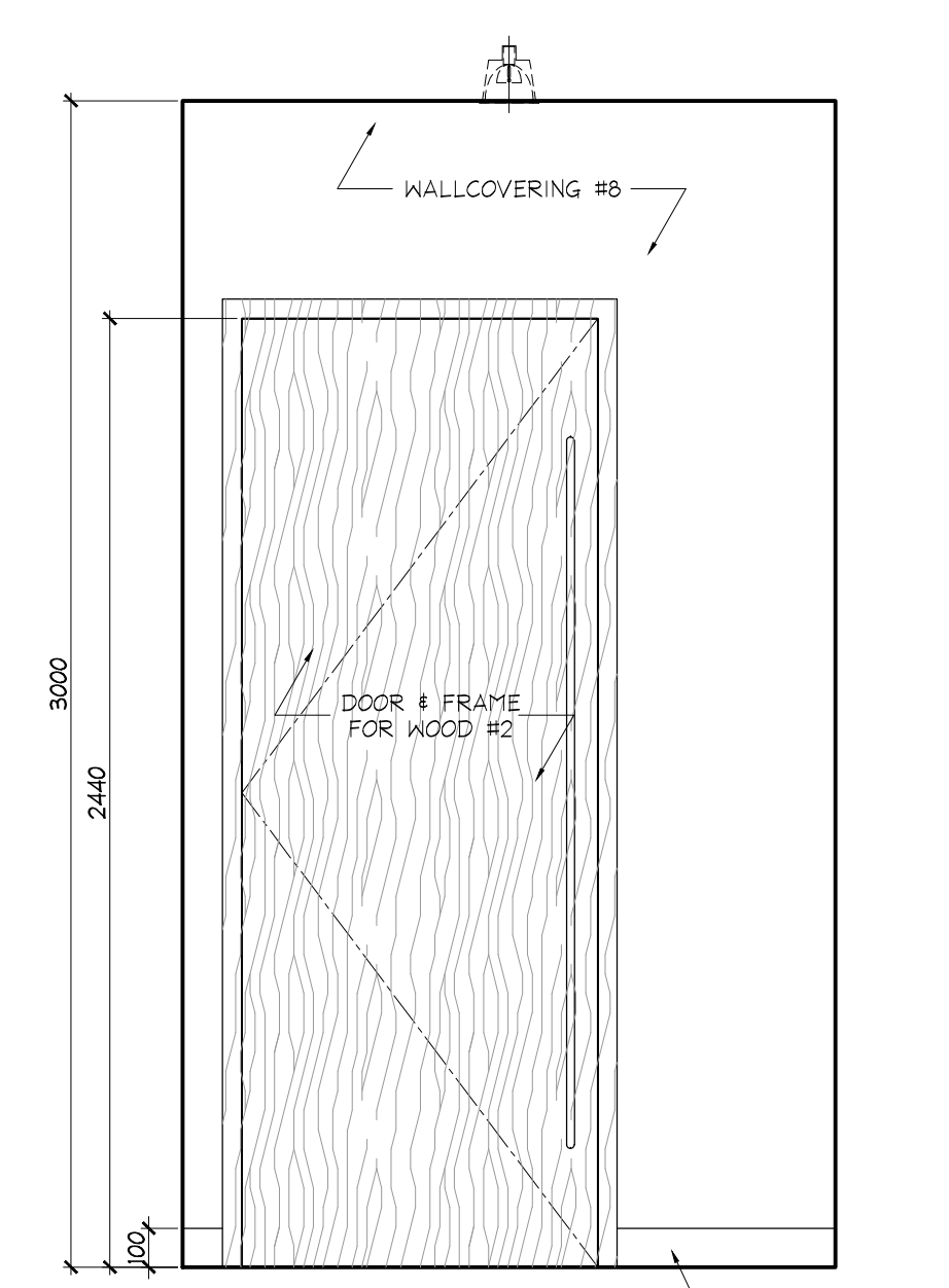
7 ELEVATION GROUND FLOOR WOMEN'S/MEN'S W.R. VESTIBULE SCALE 1:20
