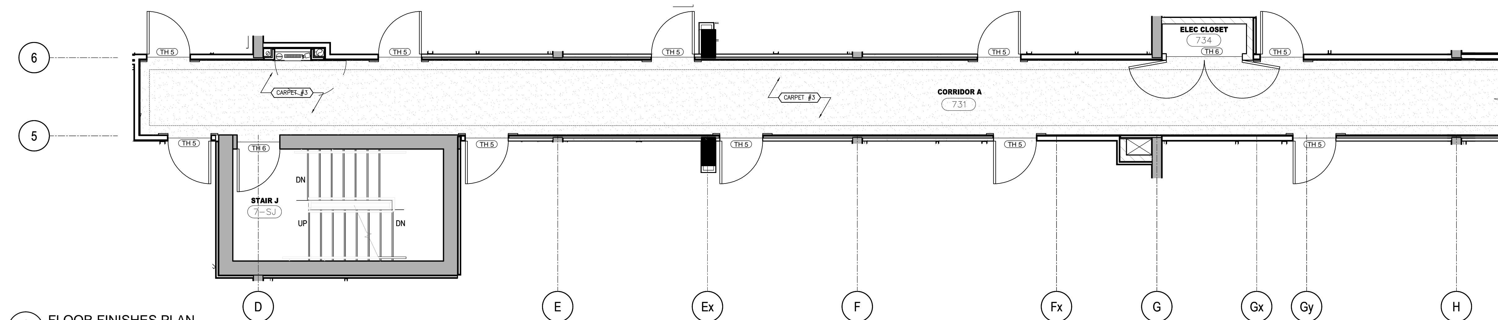
1 FLOOR FINISHES PLAN ID1.7.1 7TH FLOOR SCALE 1:50
