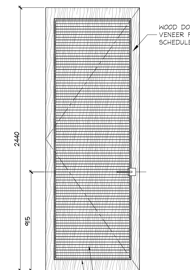
GROUND FLOOR DOORS 143B, 143C VFCU ACCESS DOOR
