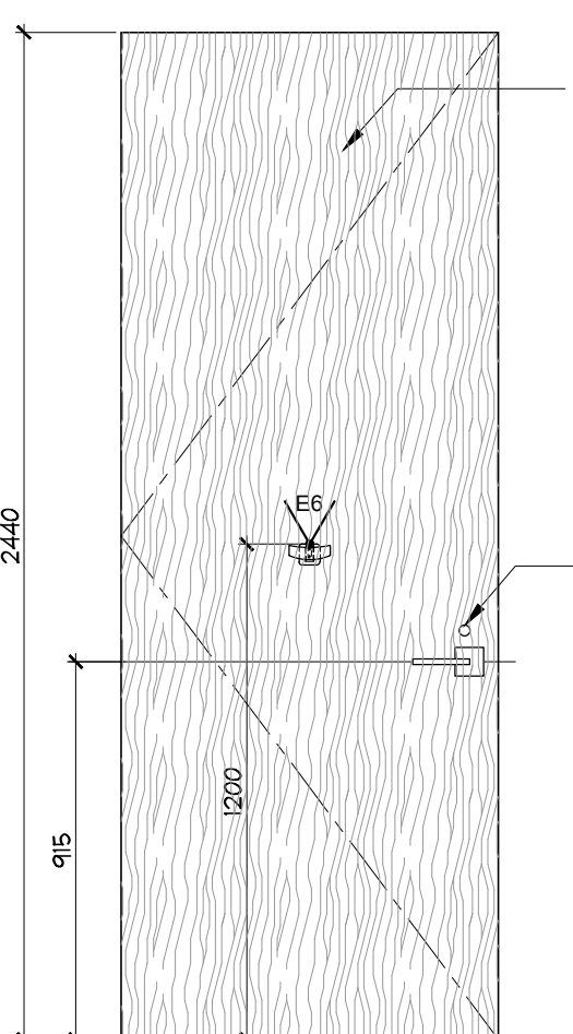
GROUND FLOOR DOORS 148, 153 (INTERIOR) MEN'S / WOMEN'S WC BF
