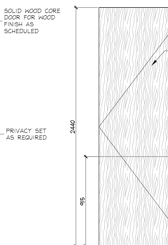
GROUND FLOOR DOOR 158 THEATRE
