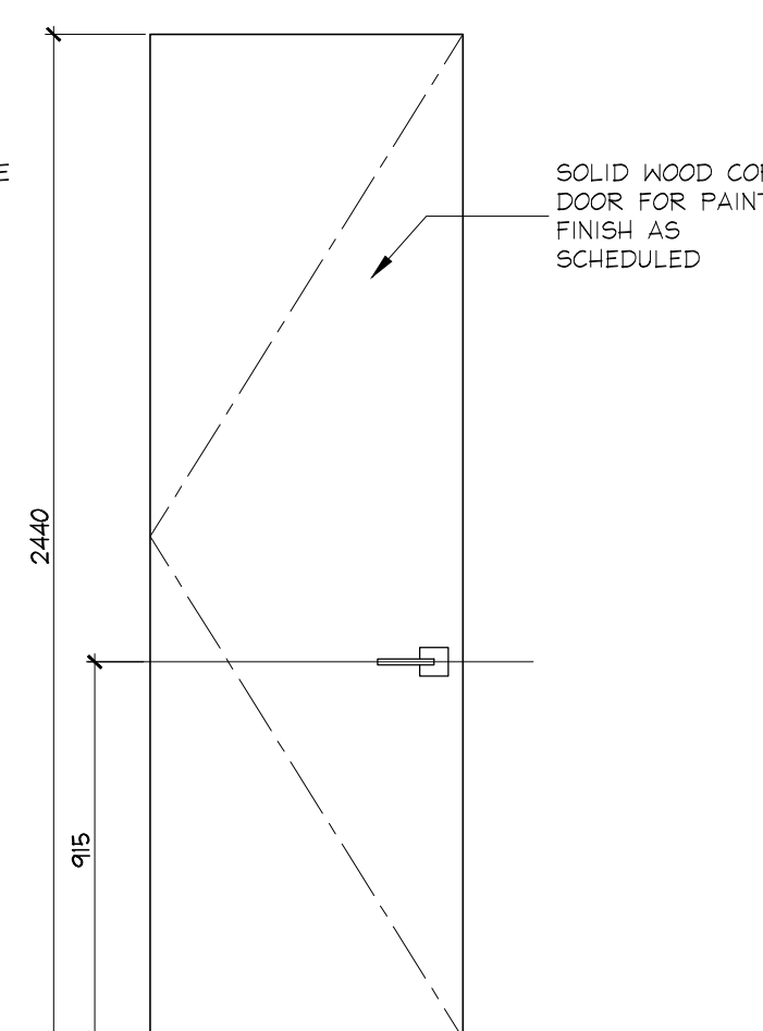
GROUND FLOOR DOOR 166.2 MANAGEMENT OFFICE (MECHANICAL CLOSET)
