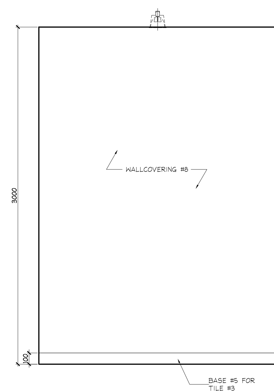
6 ELEVATION GROUND FLOOR WOMEN'S / MEN'S W.R. VESTIBULE SCALE 1:20
