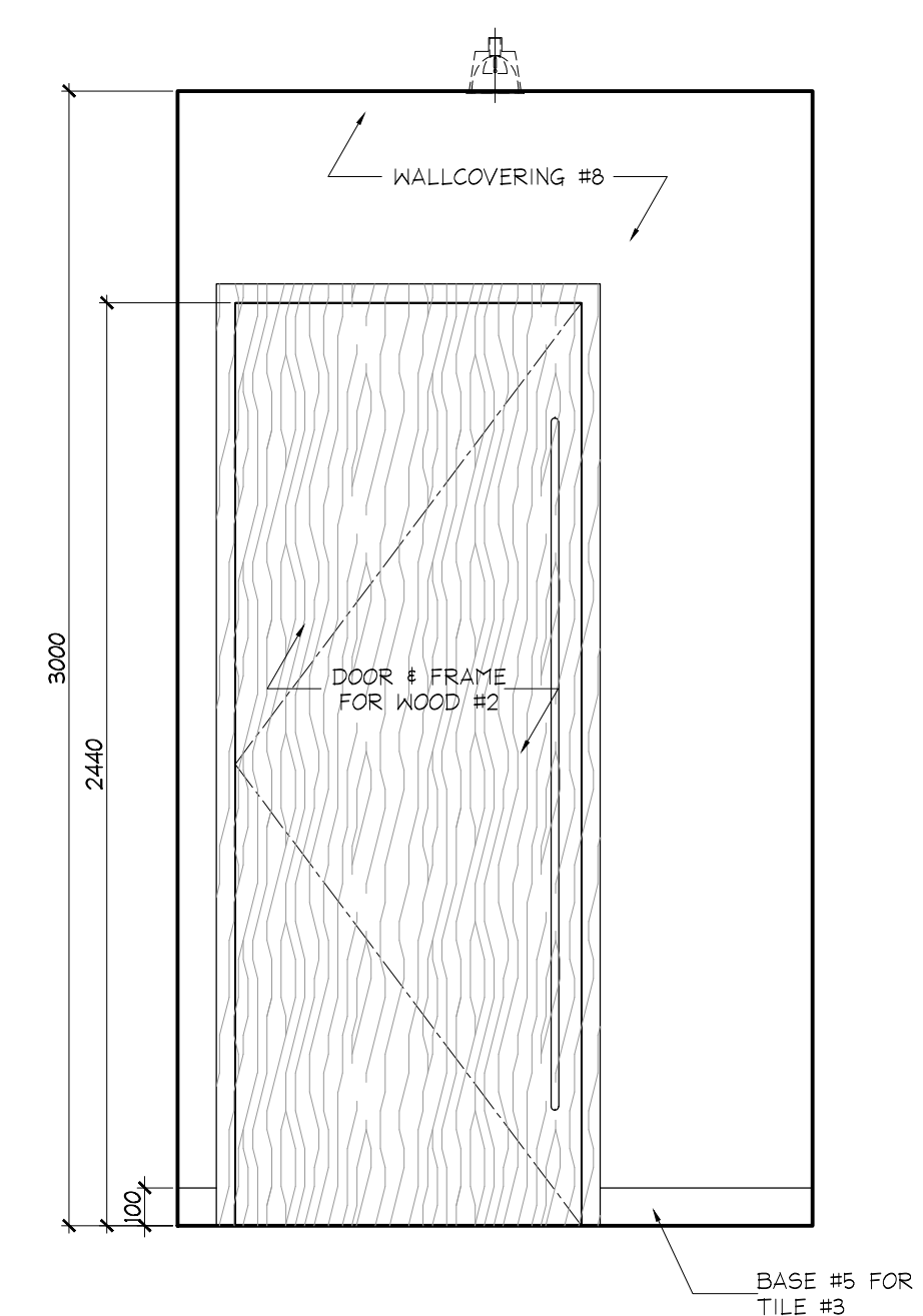
7 ELEVATION GROUND FLOOR WOMEN'S / MEN'S W.R. VESTIBULE SCALE 1:20
