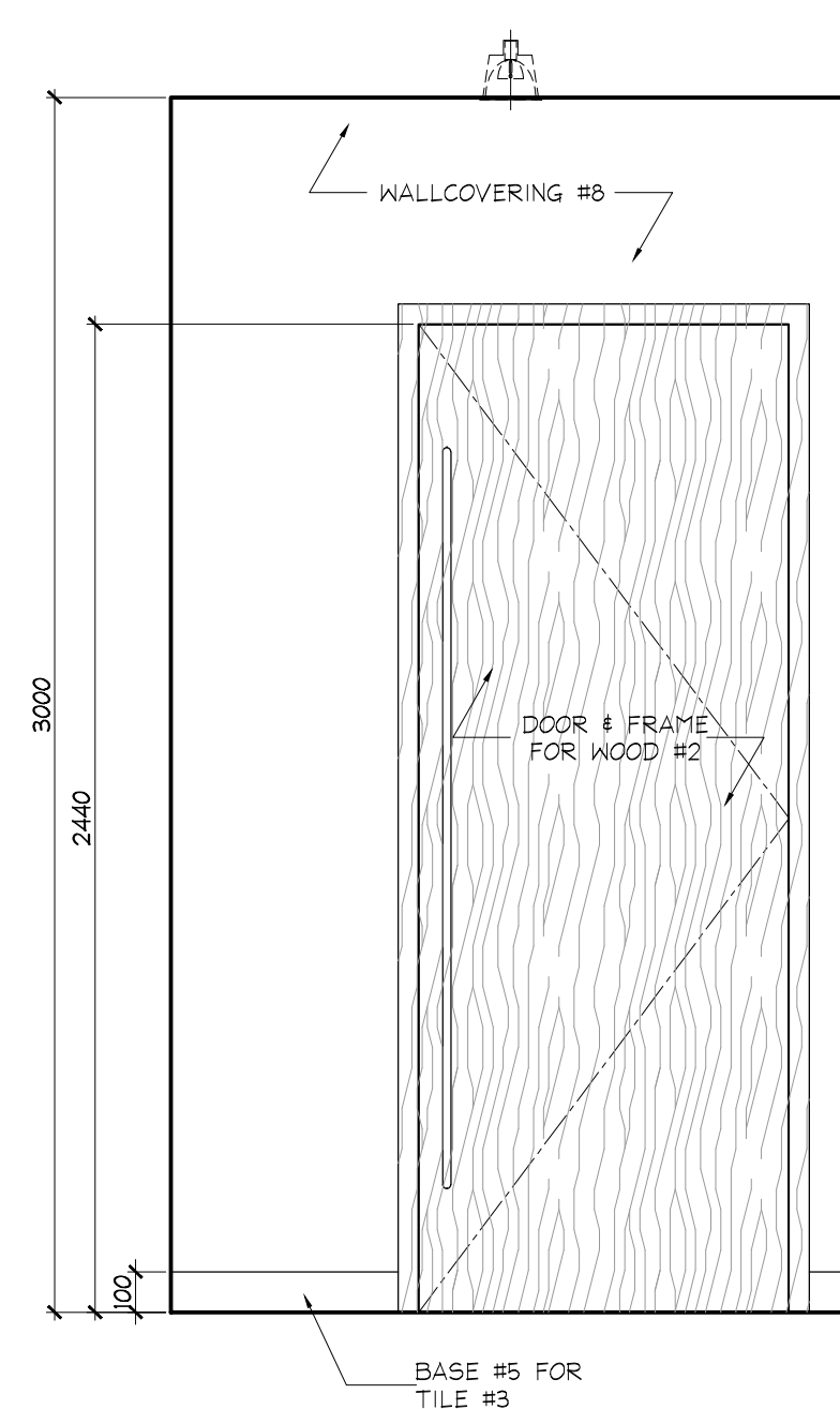
5 ELEVATION GROUND FLOOR WOMEN'S / MEN'S W.R. VESTIBULE SCALE 1:20
