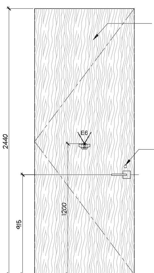
GROUND FLOOR DOORS 148, 153 (INTERIOR) MEN'S / WOMEN'S WC BF
