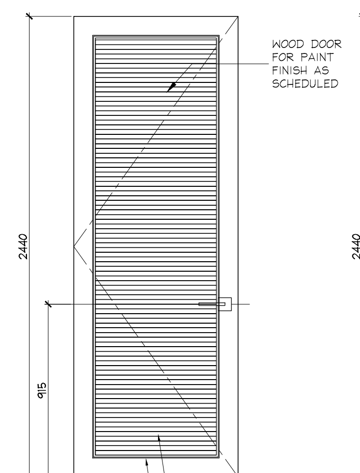
GROUND FLOOR DOORS 162A, 163A VFCU ACCESS DOOR
