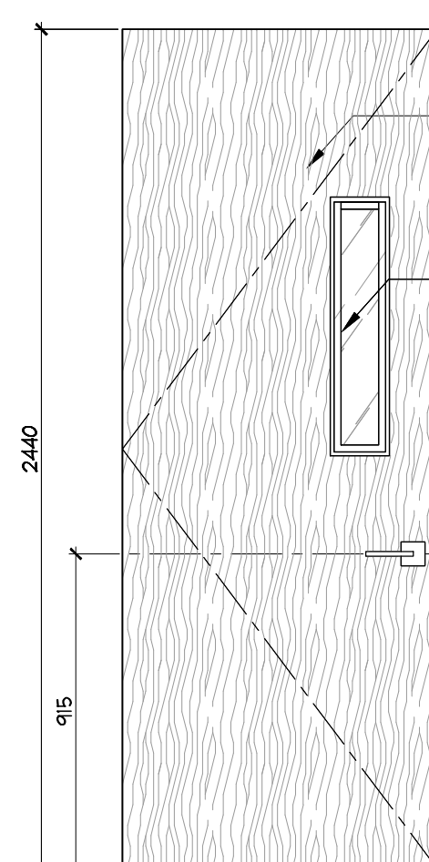
GROUND FLOOR DOOR 160.1 CORRIDOR C TO CORRIDOR A
