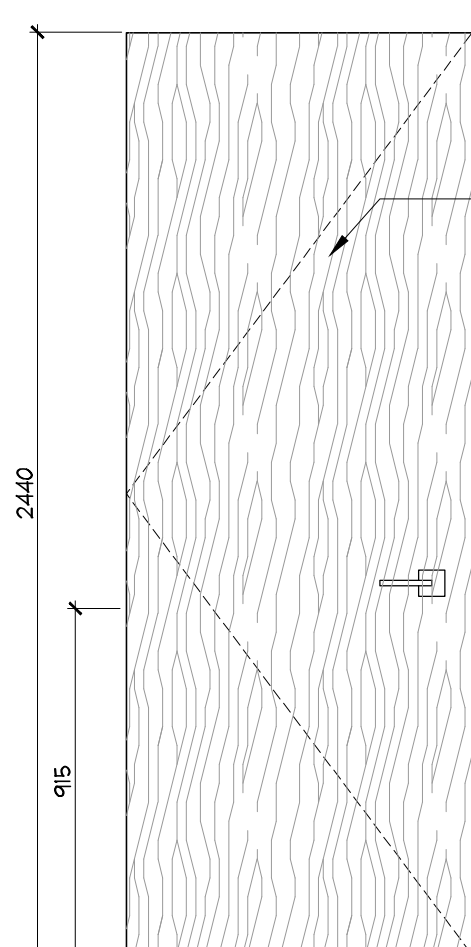
GROUND FLOOR DOORS 161.1, 161.2 DINING ROOM
