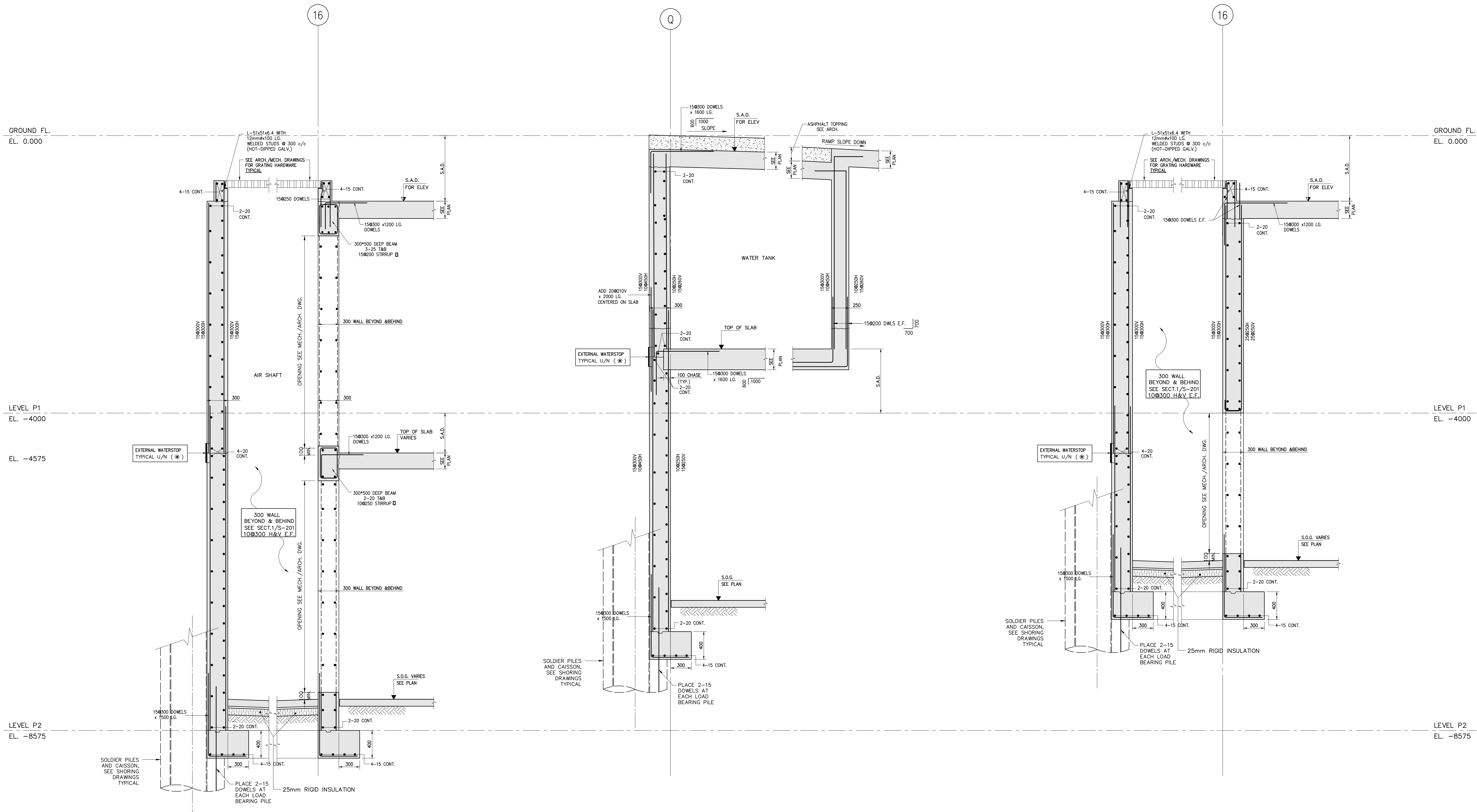
SECTION 1 SCALE 1:20
