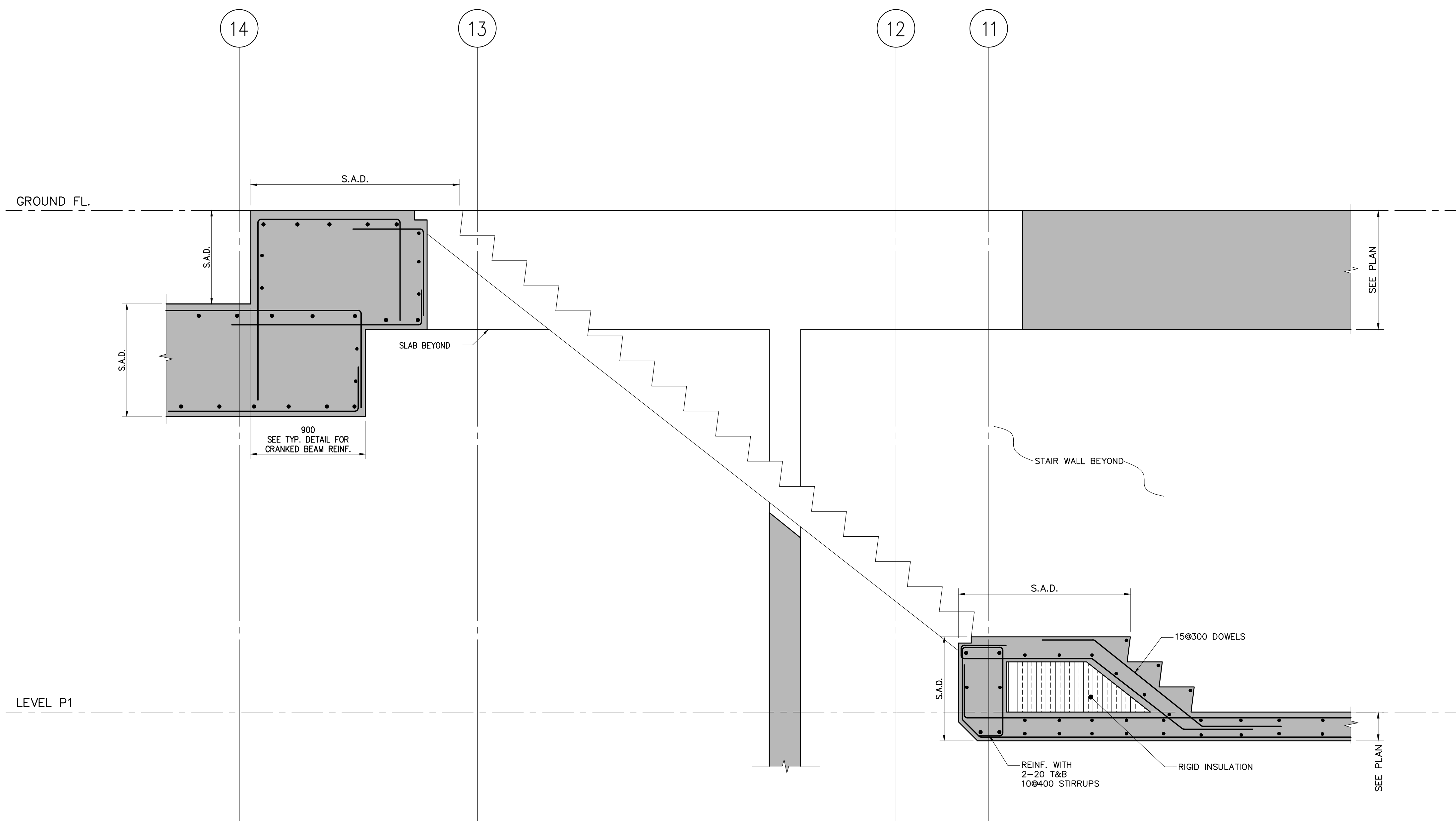
SECTION 1 SCALE 1:20 S-308
