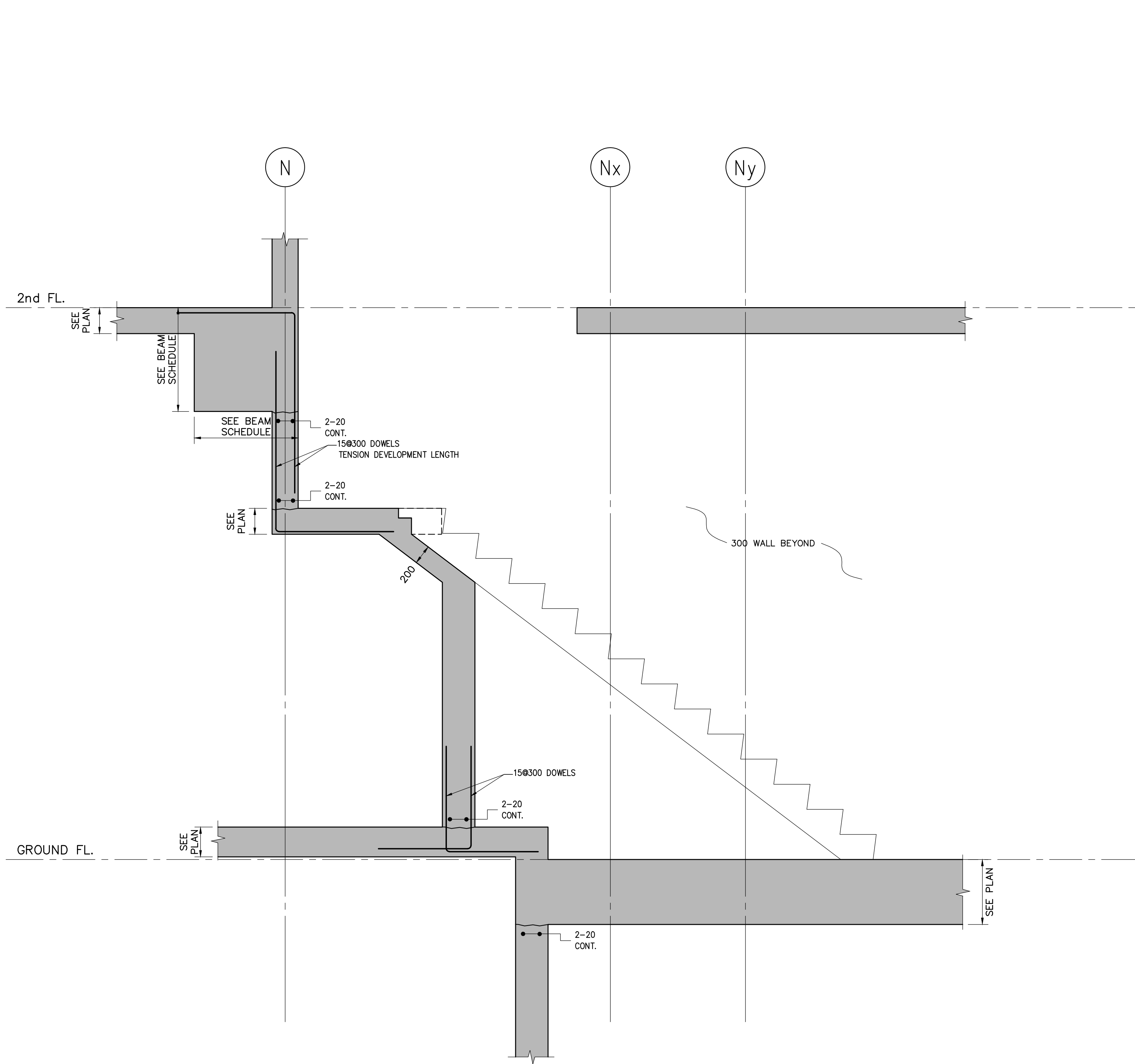
SECTION 2 SCALE 1:20 S-308
