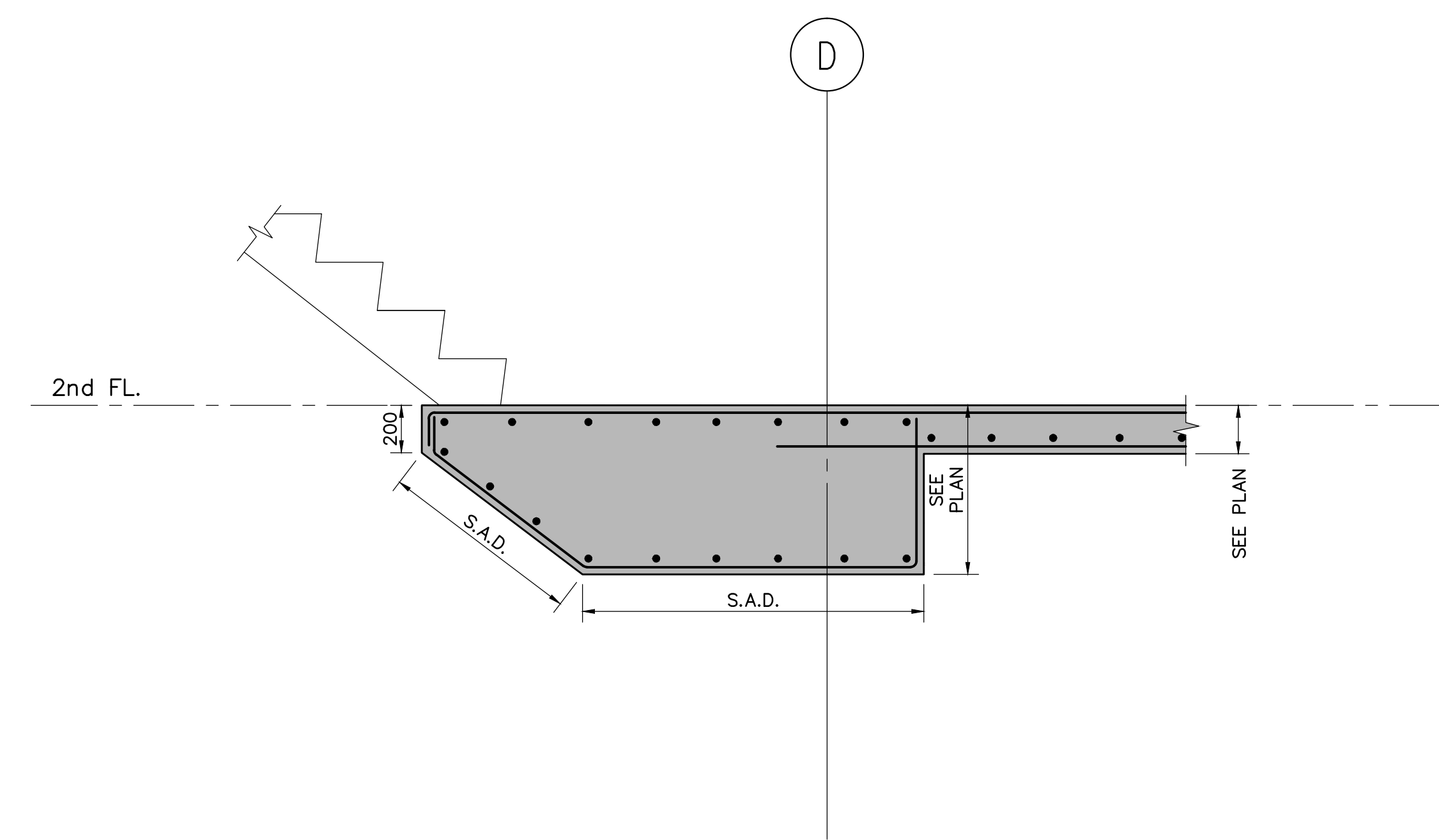
SECTION 4 SCALE 1:20 S-308
