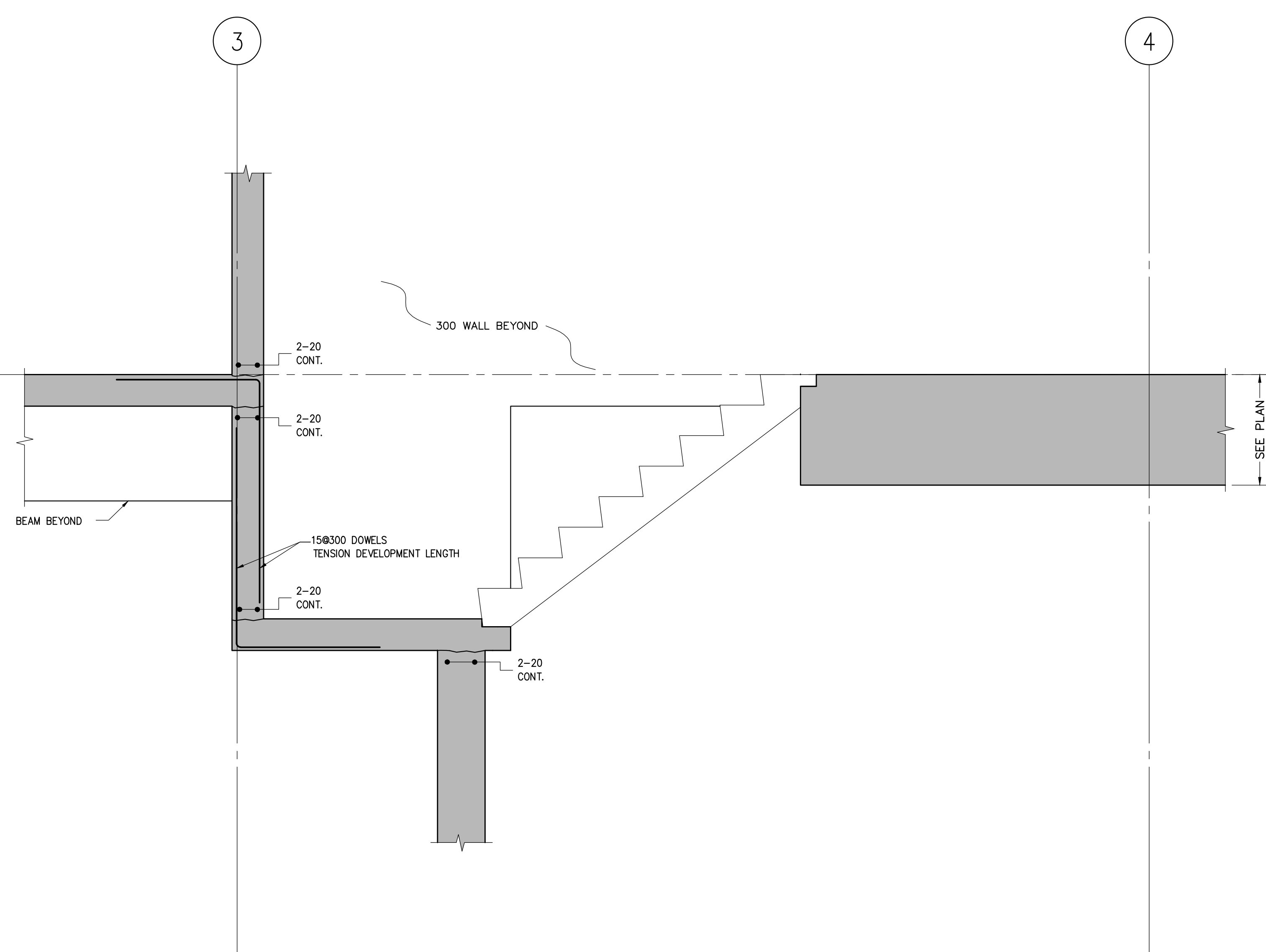
SECTION 3 SCALE 1:20 S-308
