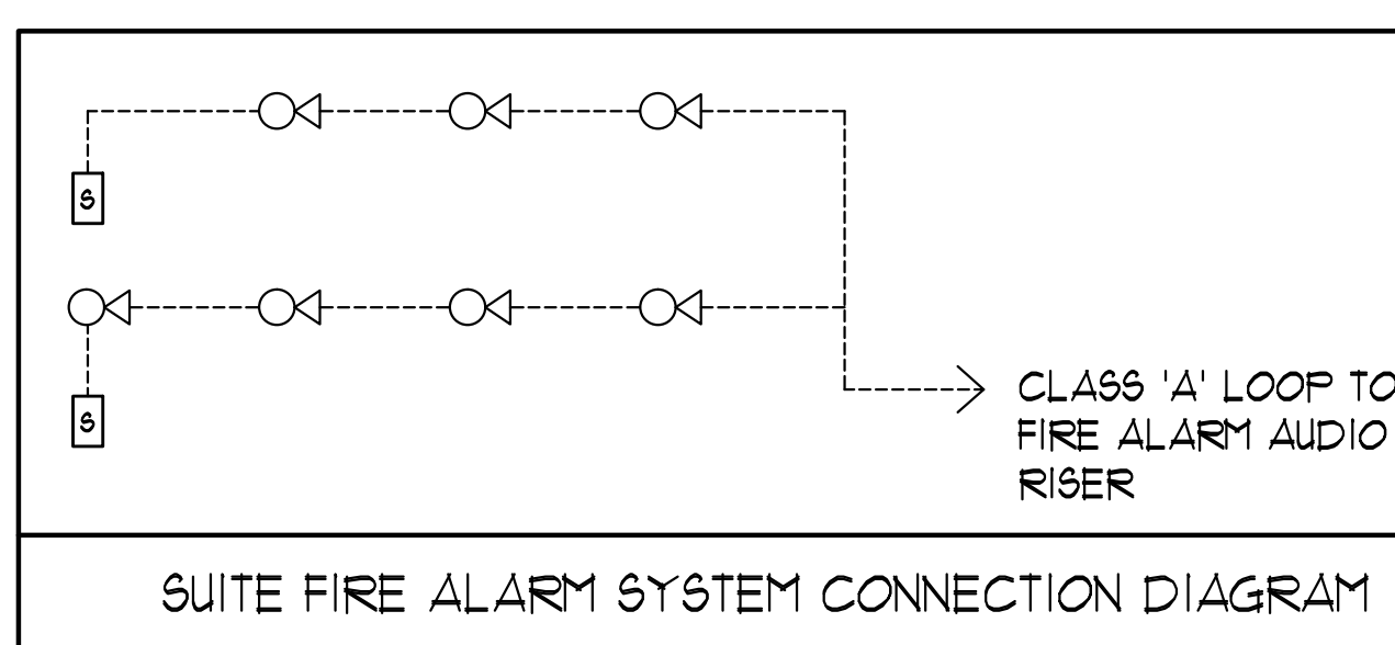
SUITE FIRE ALARM SYSTEM CONNECTION DIAGRAM
