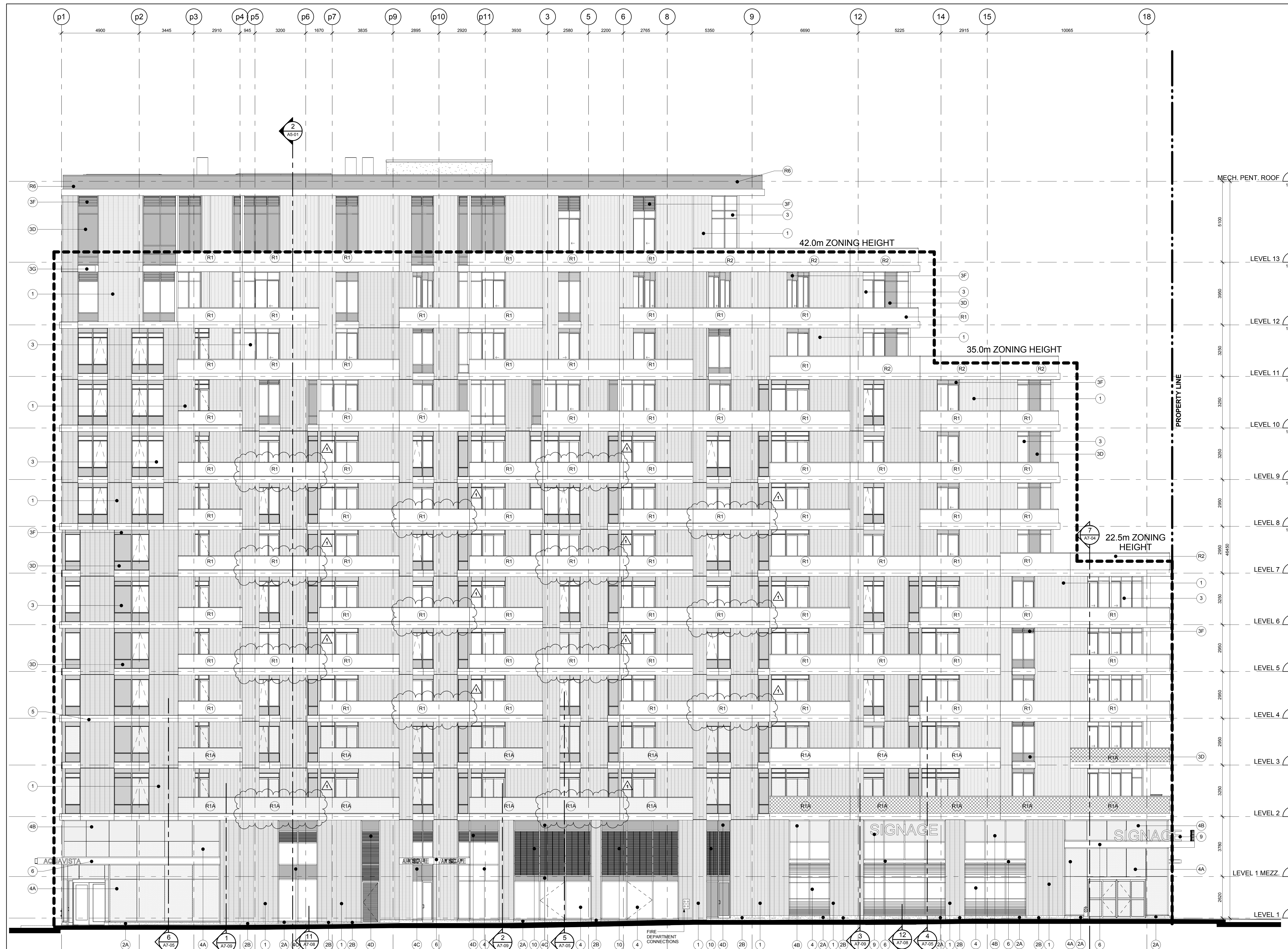
West Elevation 2 A4-02
