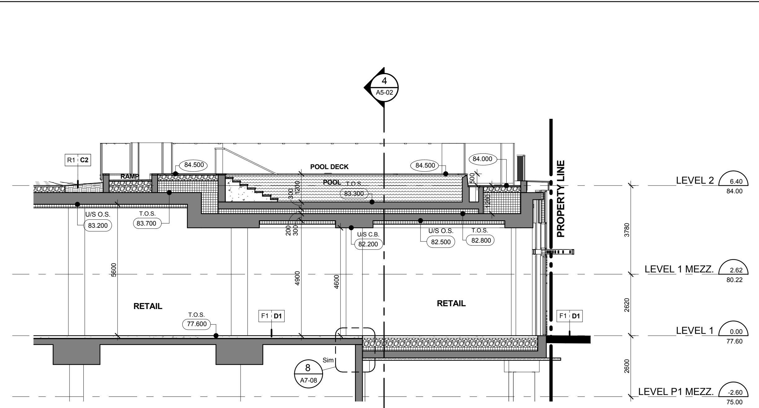
North - South Pool Section Along Gridline J
