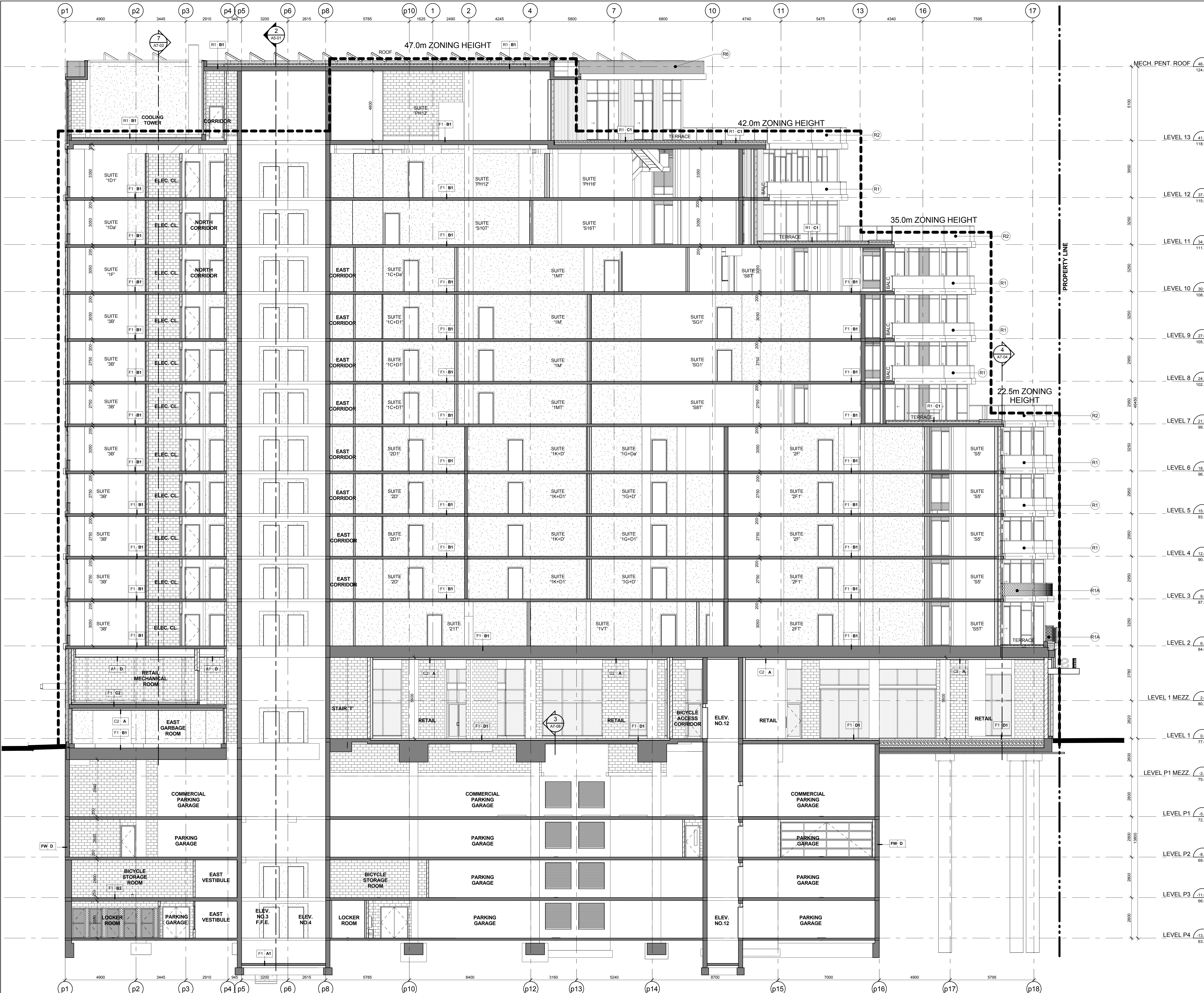
North - South Building Section Along Gridline pP
