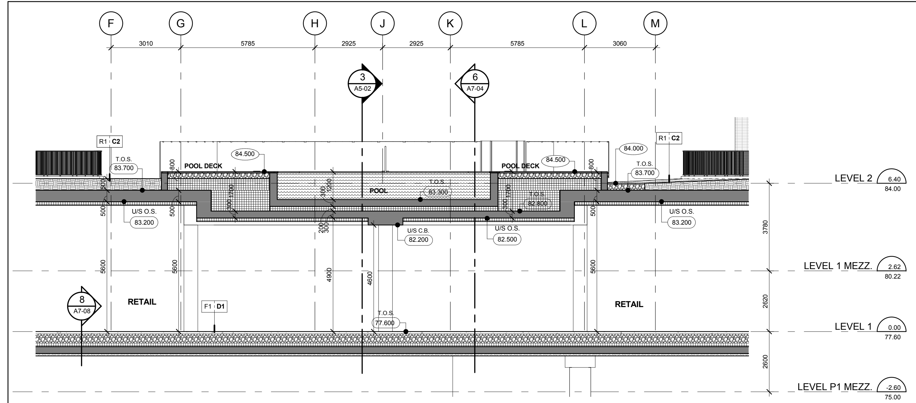
East - West Pool Section Along Gridline p17
