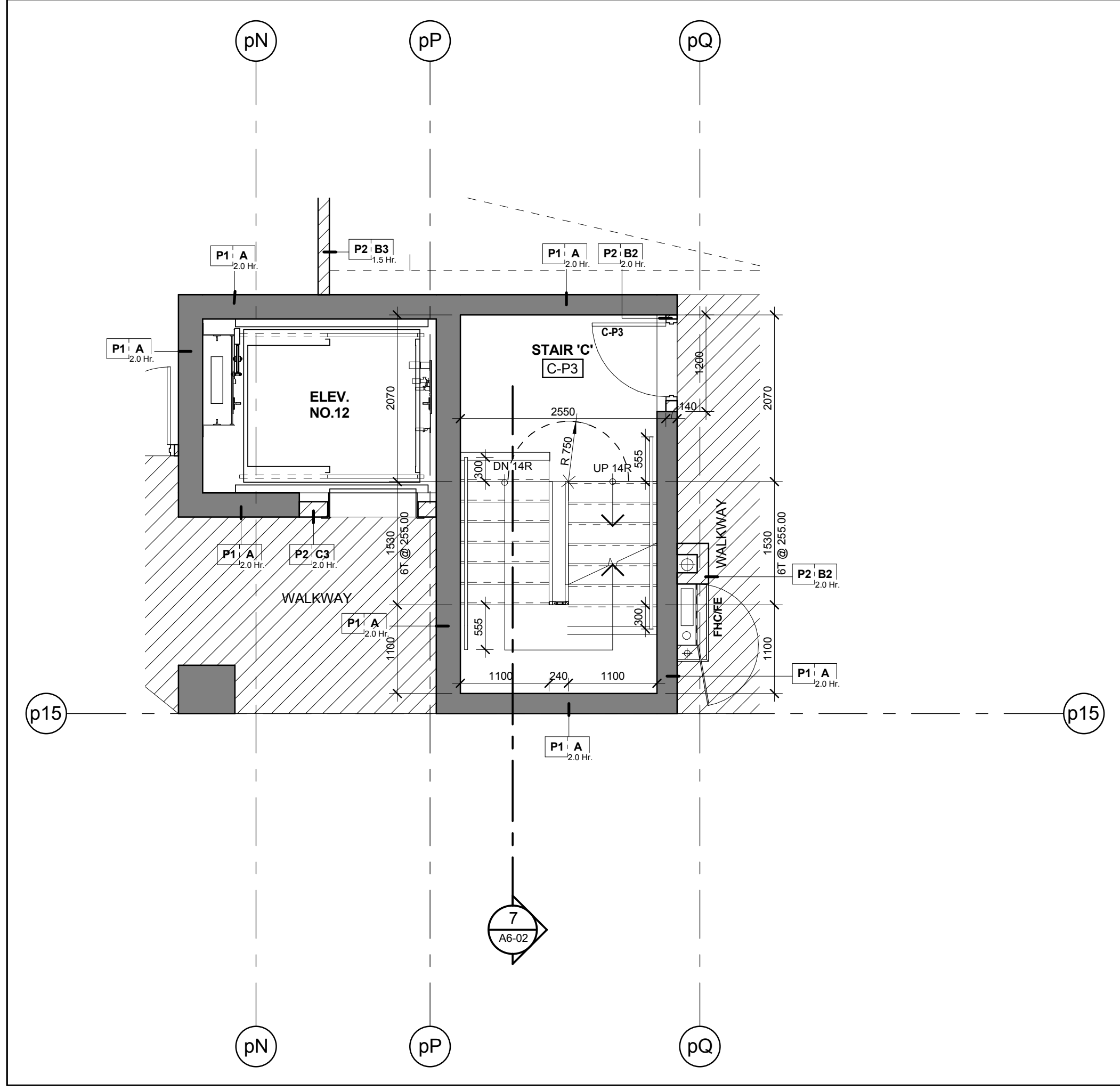
Stair 'C' - Stair Plan - Level P3 2 Scale: 1 : 50 A6-02
