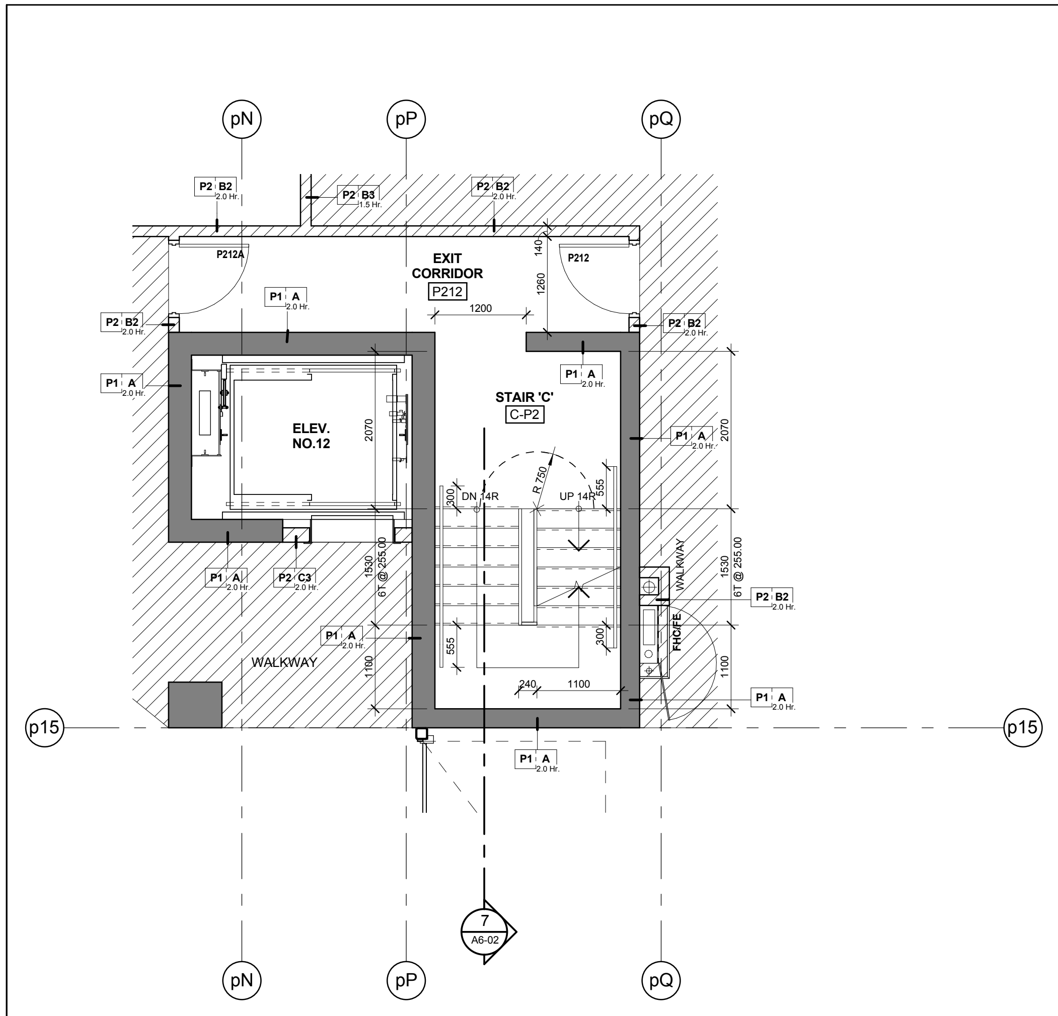
Stair 'C' - Stair Plan - Level P2 3 Scale: 1 : 50 A6-02
