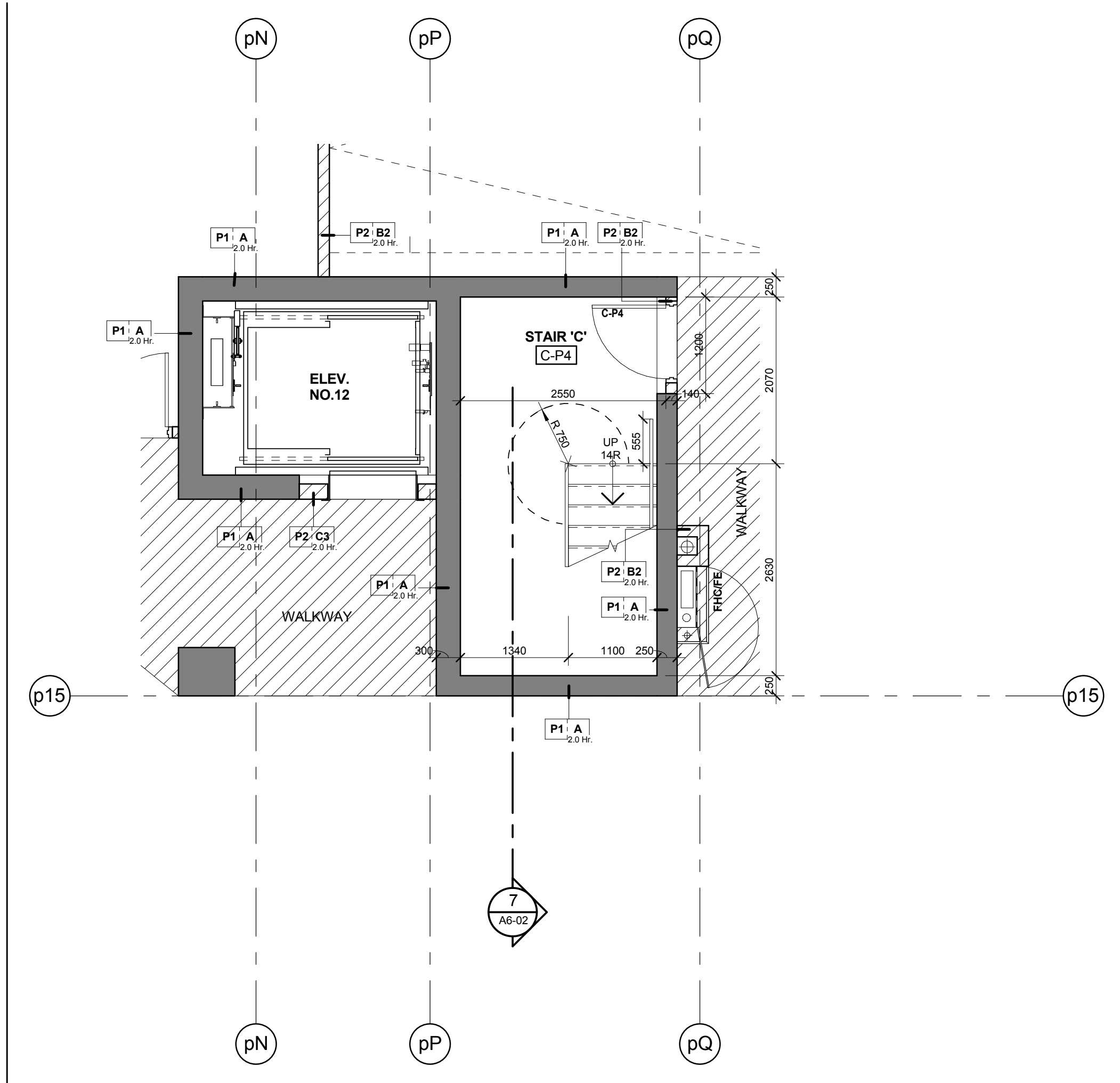
Stair 'C' - Stair Plan - Level P4 1 Scale: 1 : 50 A6-02
