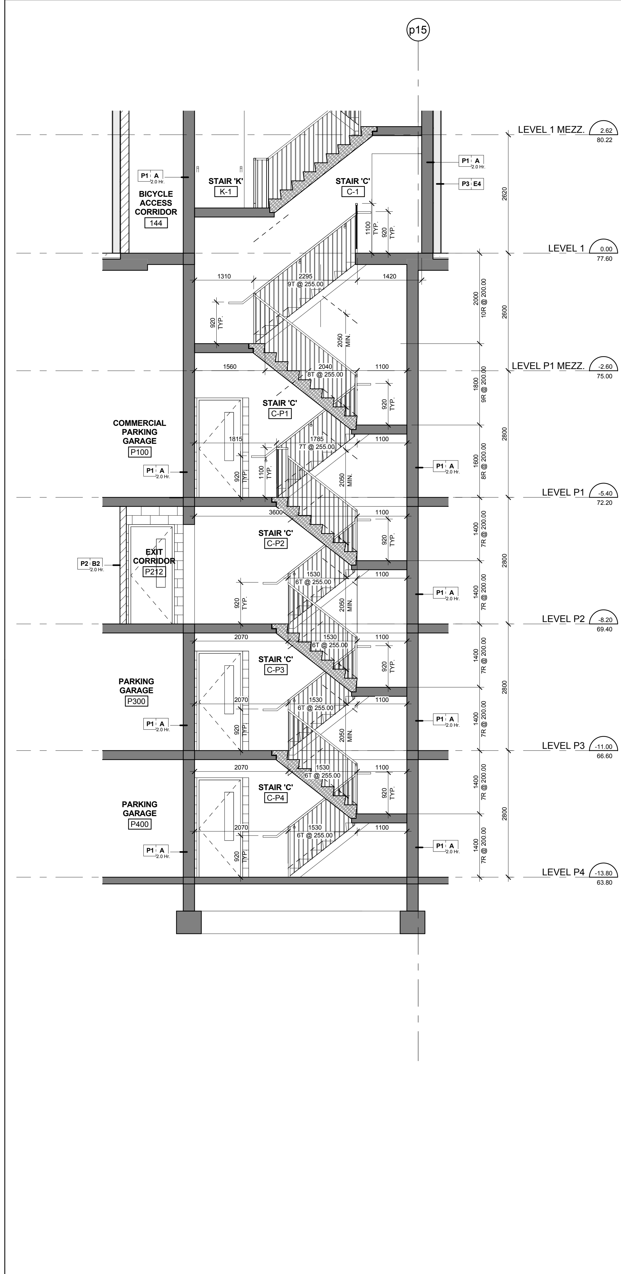
Stair 'C' - Stair Section Levels P4 - 1 Mezzanine 7 Scale: 1 : 50 A6-02
