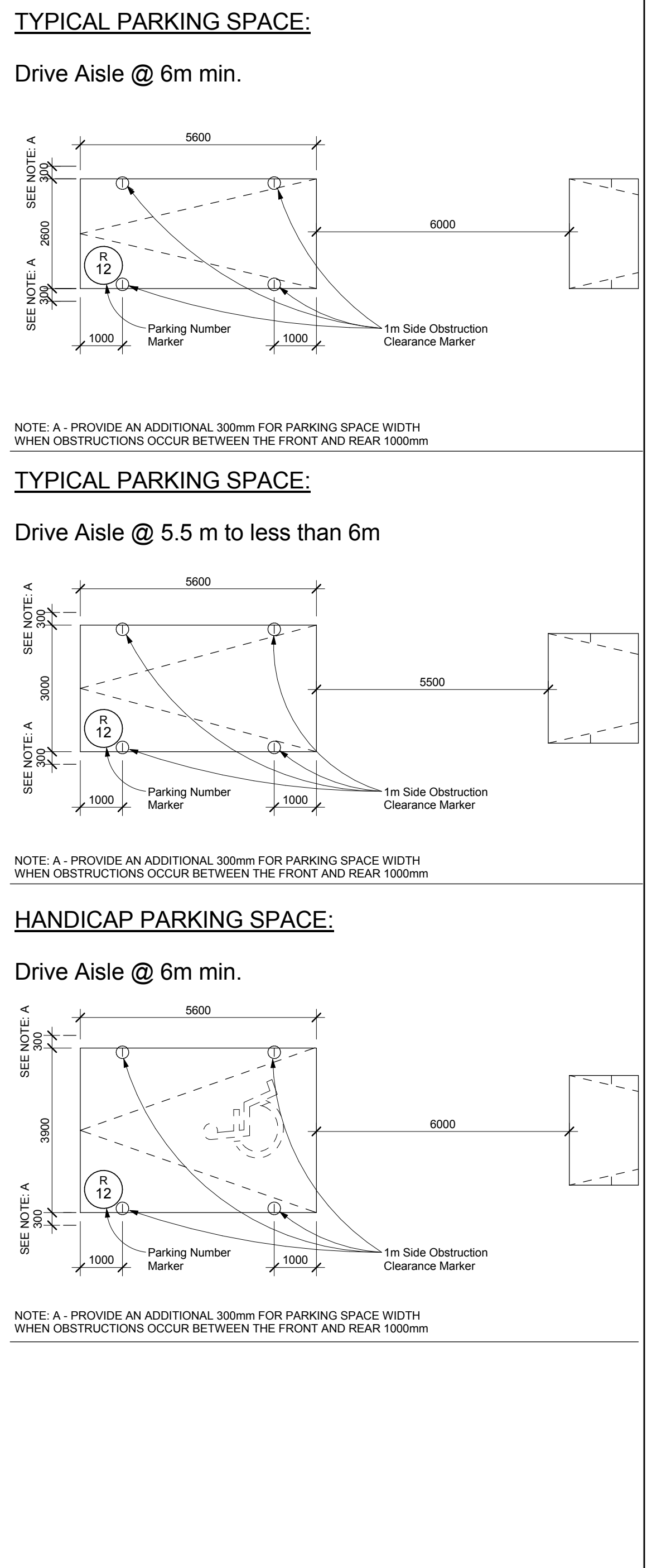
Typical Parking Space Legend 4 A2-04
