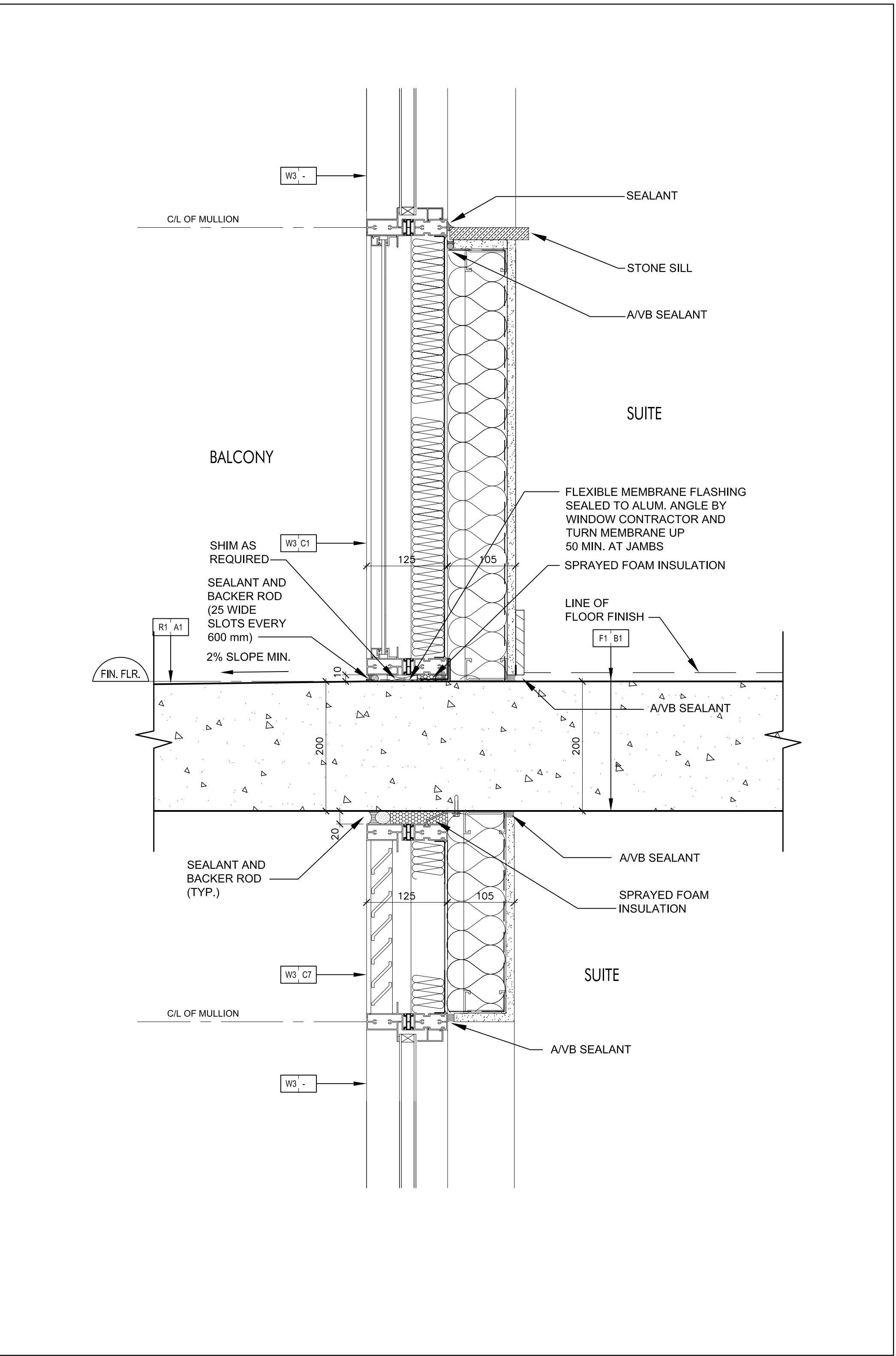
Window Wall @ Balcony 9 SCALE 1:5 A7-11
