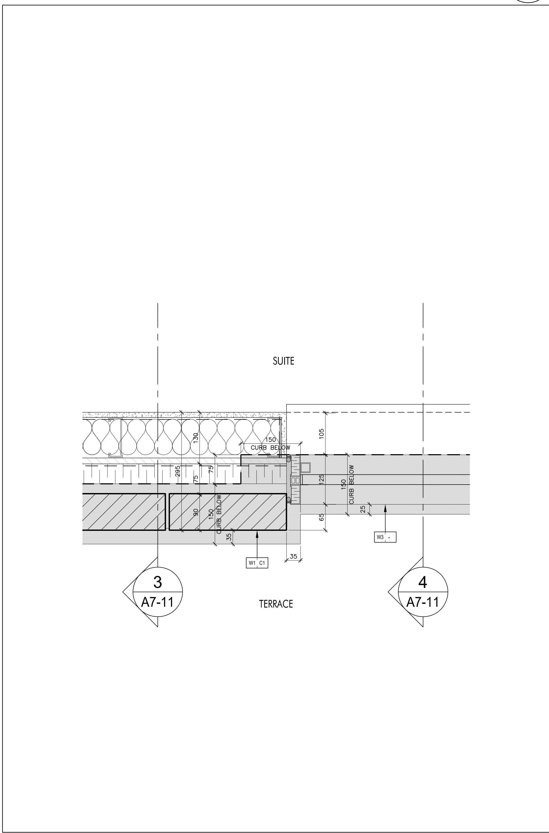
Plan Detail of Window Wall & Brick Wall @ Terrace 5 SCALE 1:5 A7-11
