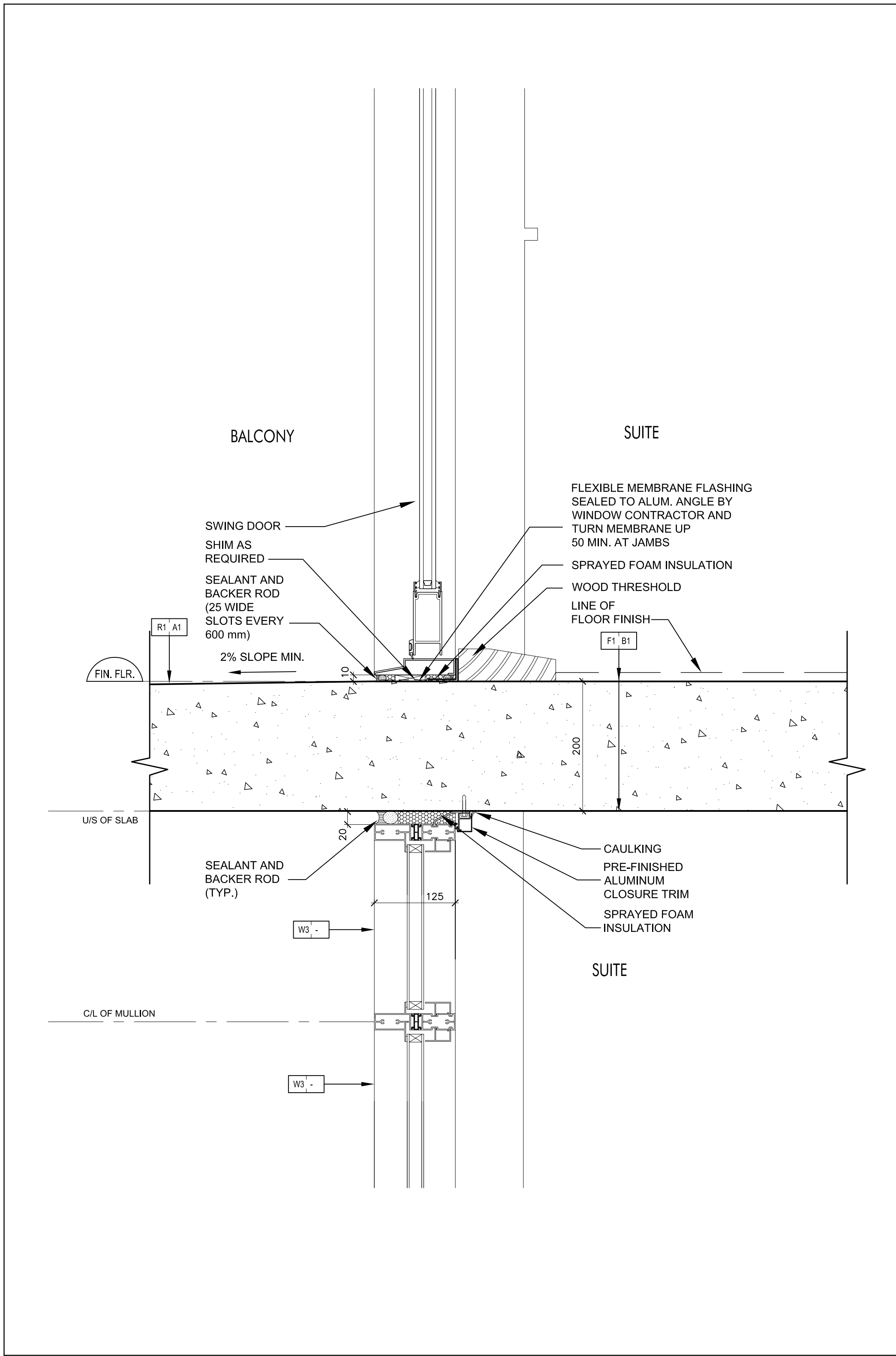
Swing Door @ Balcony 11 SCALE 1:5 A7-11
