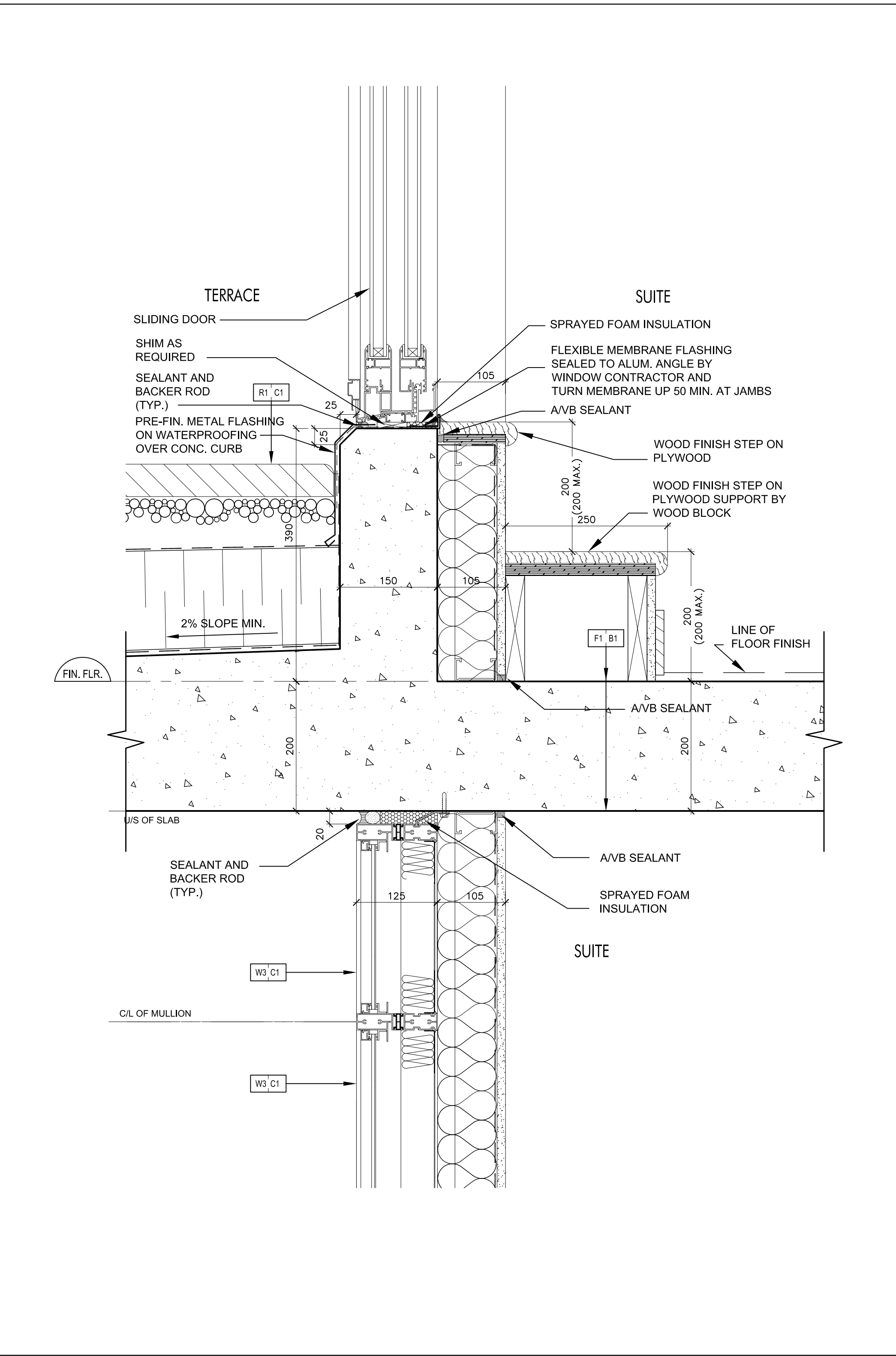
Sliding Door @ Terrace 7 SCALE 1:5 A7-11
