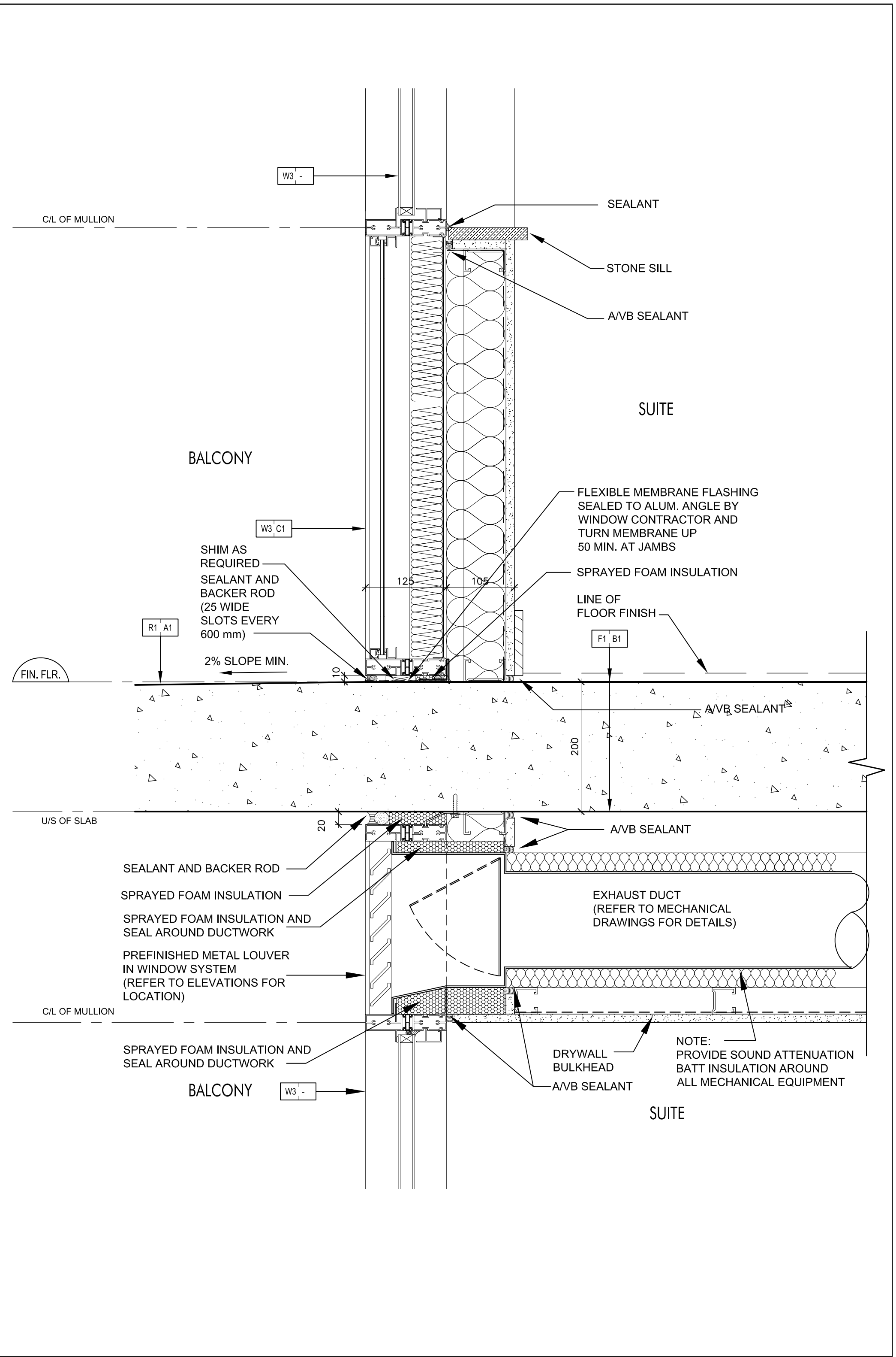
Window Wall @ Balcony 8 SCALE 1:5 A7-11
