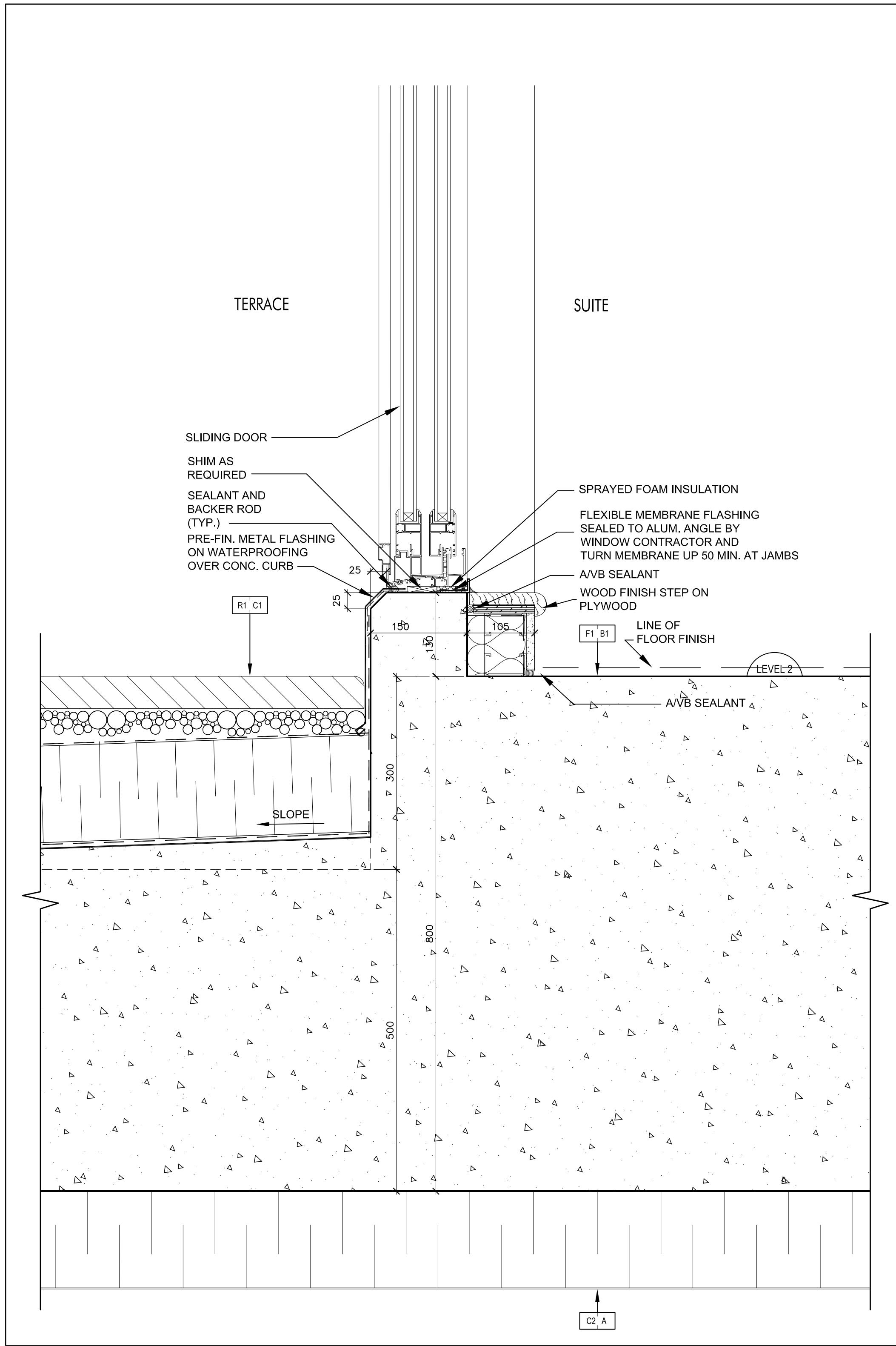
Concrete Curb @ Sliding Door @ Terrace @ Level 2 12 SCALE 1:5 A7-11
