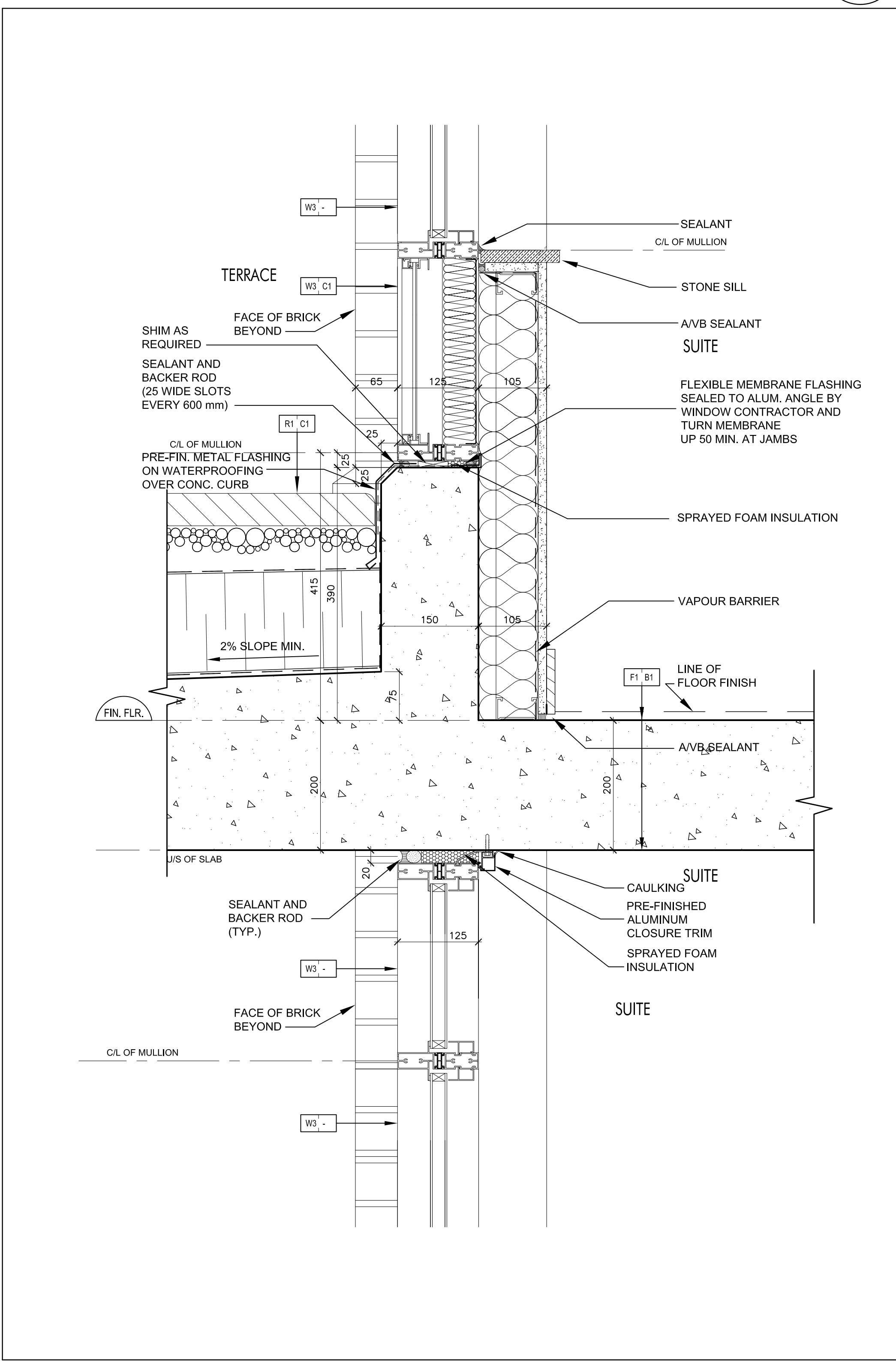
Window Wall @ Terrace 4 SCALE 1:5 A7-11
