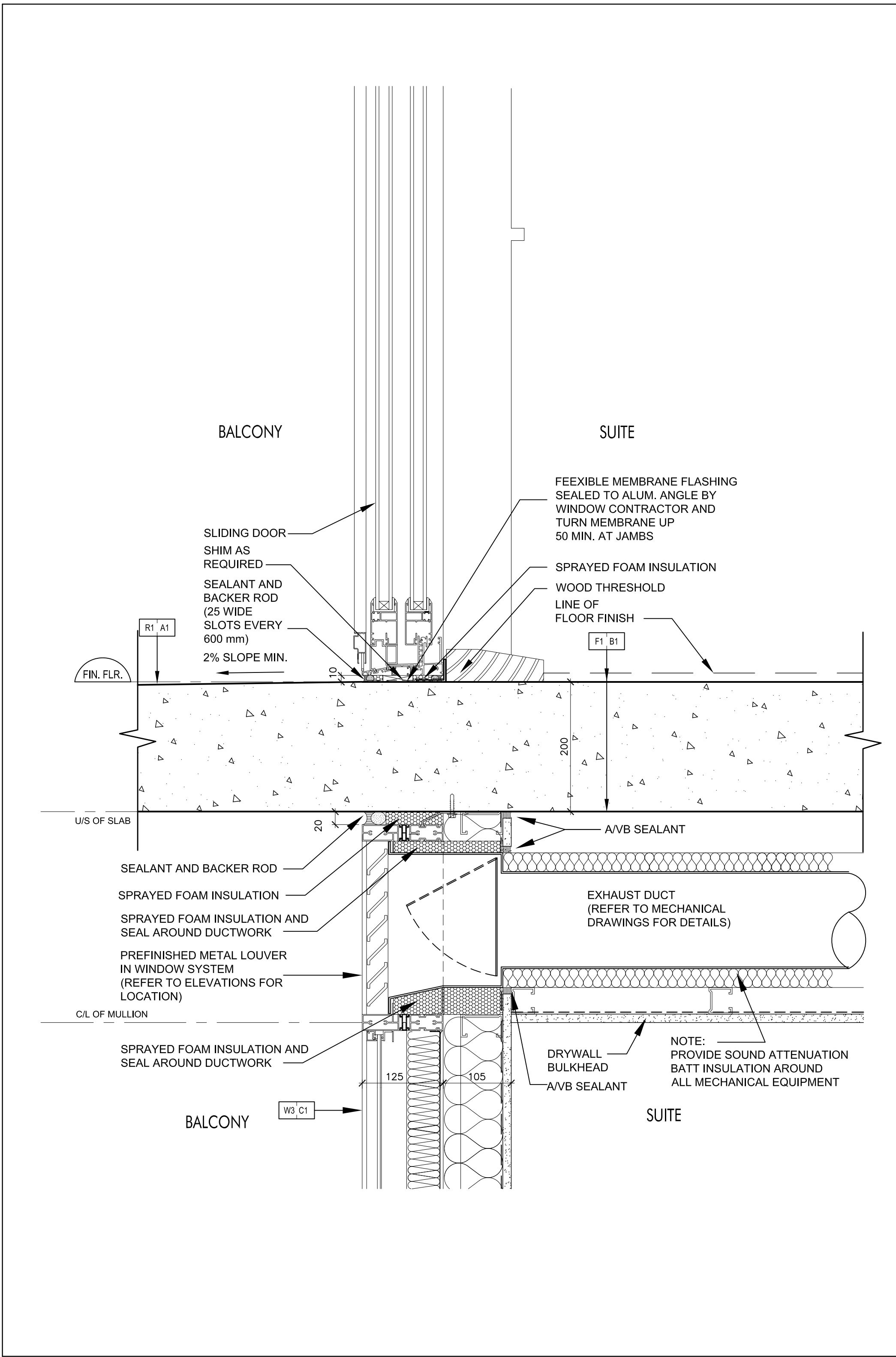
Sliding Door @ Balcony 10 SCALE 1:5 A7-11
