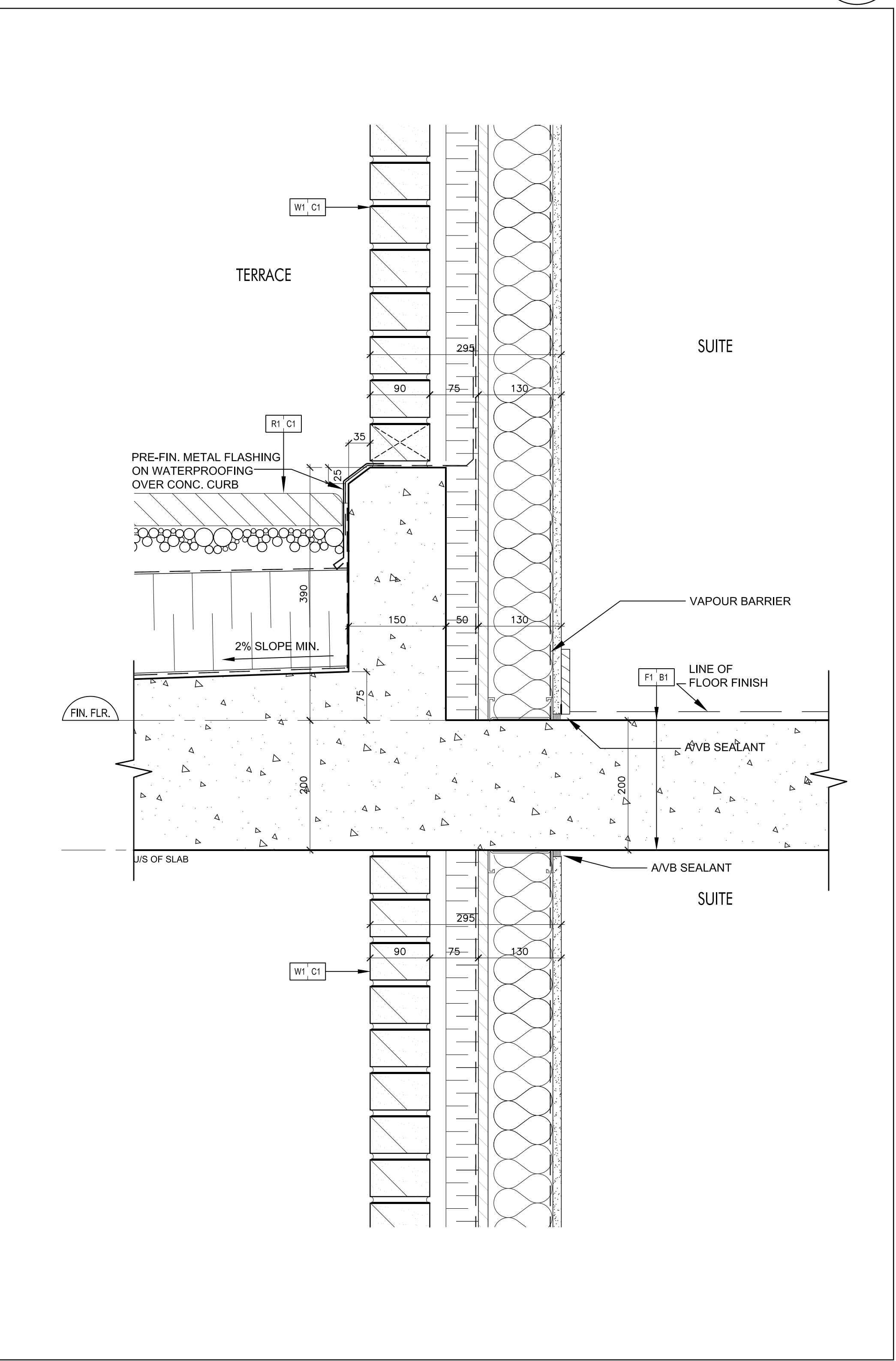
Brick Wall @ Terrace 3 SCALE 1:5 A7-11
