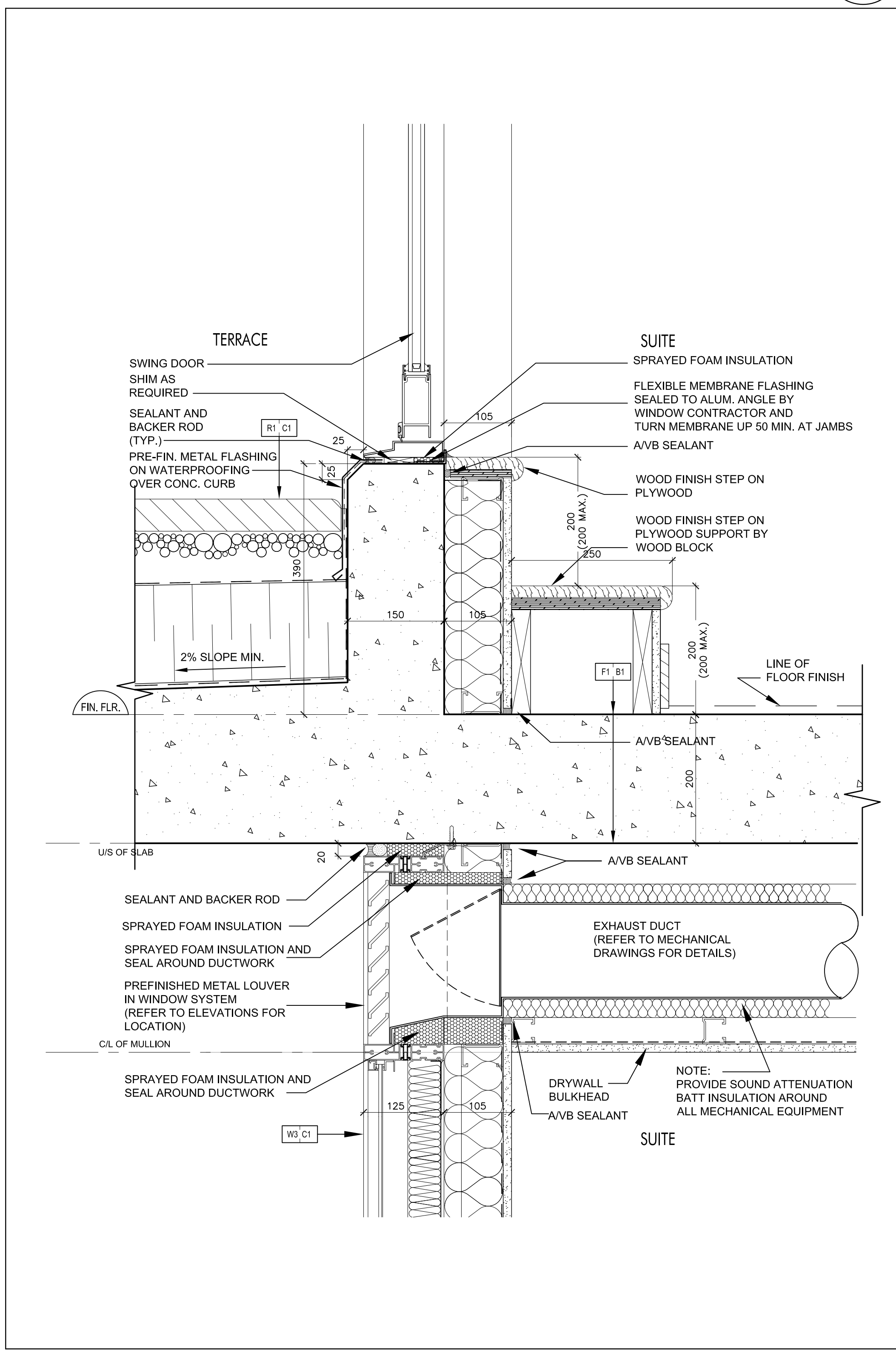
Swing Door @ Terrace 6 SCALE 1:5 A7-11
