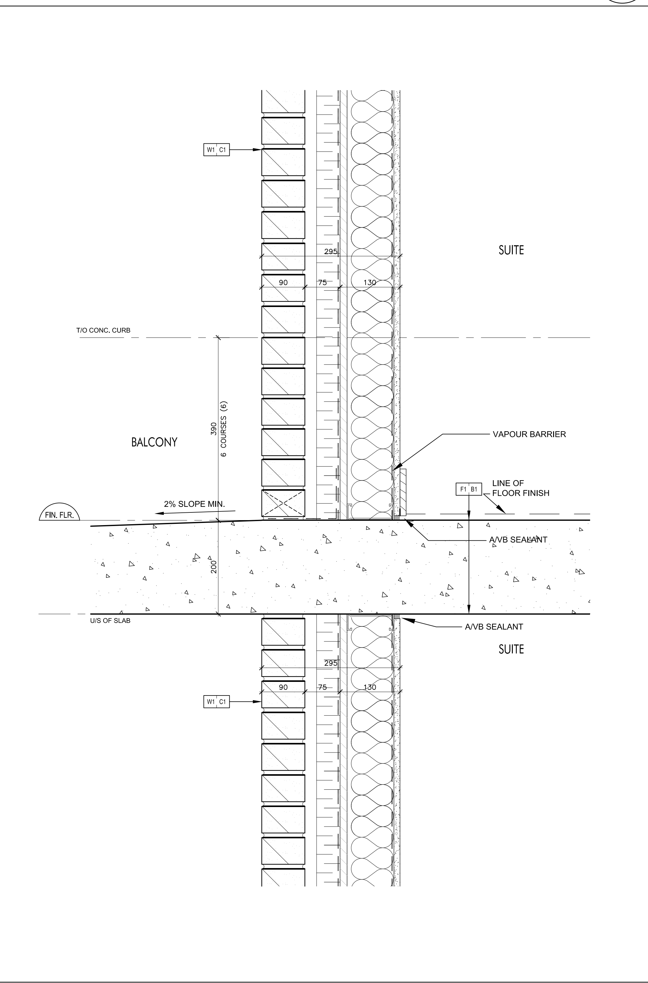
Brick Wall @ Balcony 1 SCALE 1:5 A7-11
