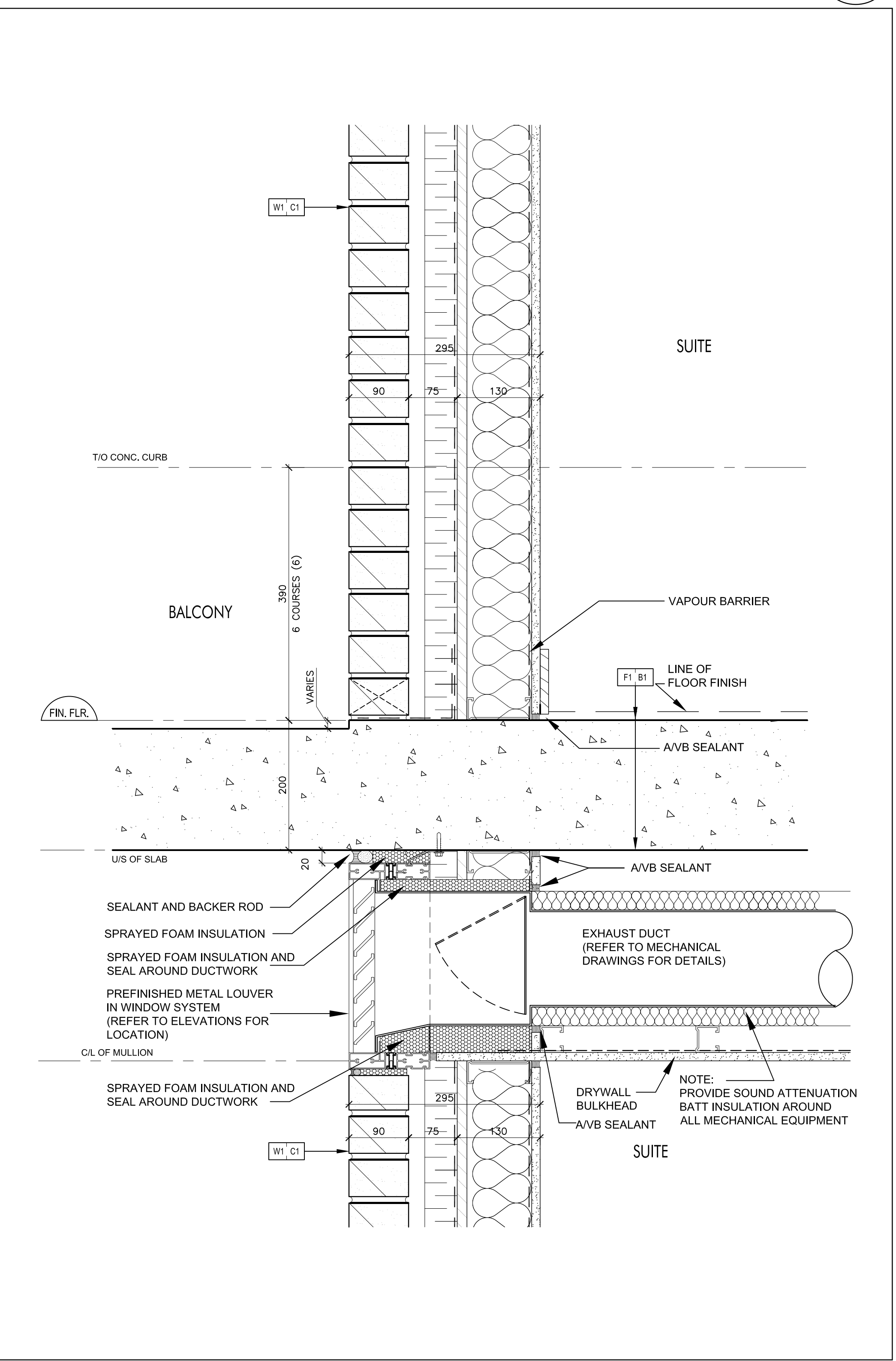
Brick Wall @ Balcony 2 SCALE 1:5 A7-11
