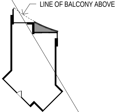
BALCONY PLAN: FLOORS 4, 6 2D1
