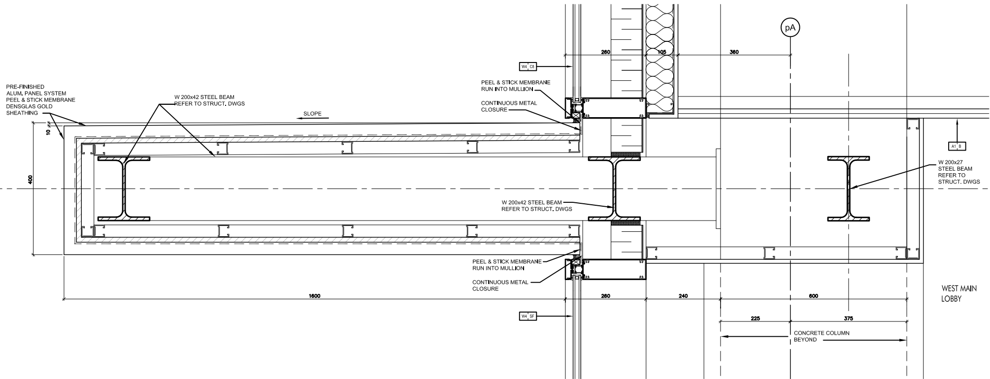
Pre-Finished Aluminum Canopy @ West Main Lobby @ Level 1
