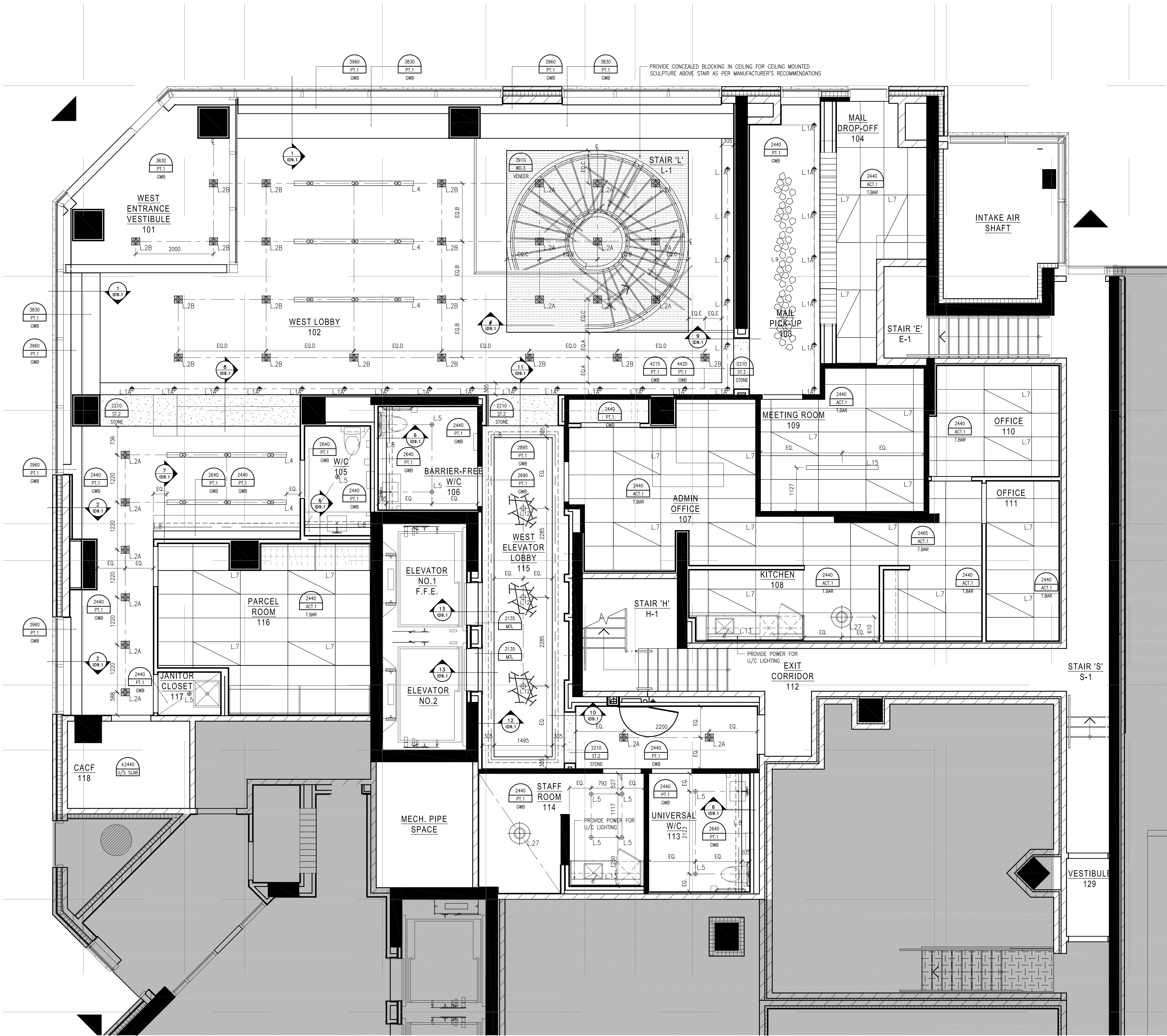
1 REFLECTED CEILING PLAN SCALE: 1/16"
