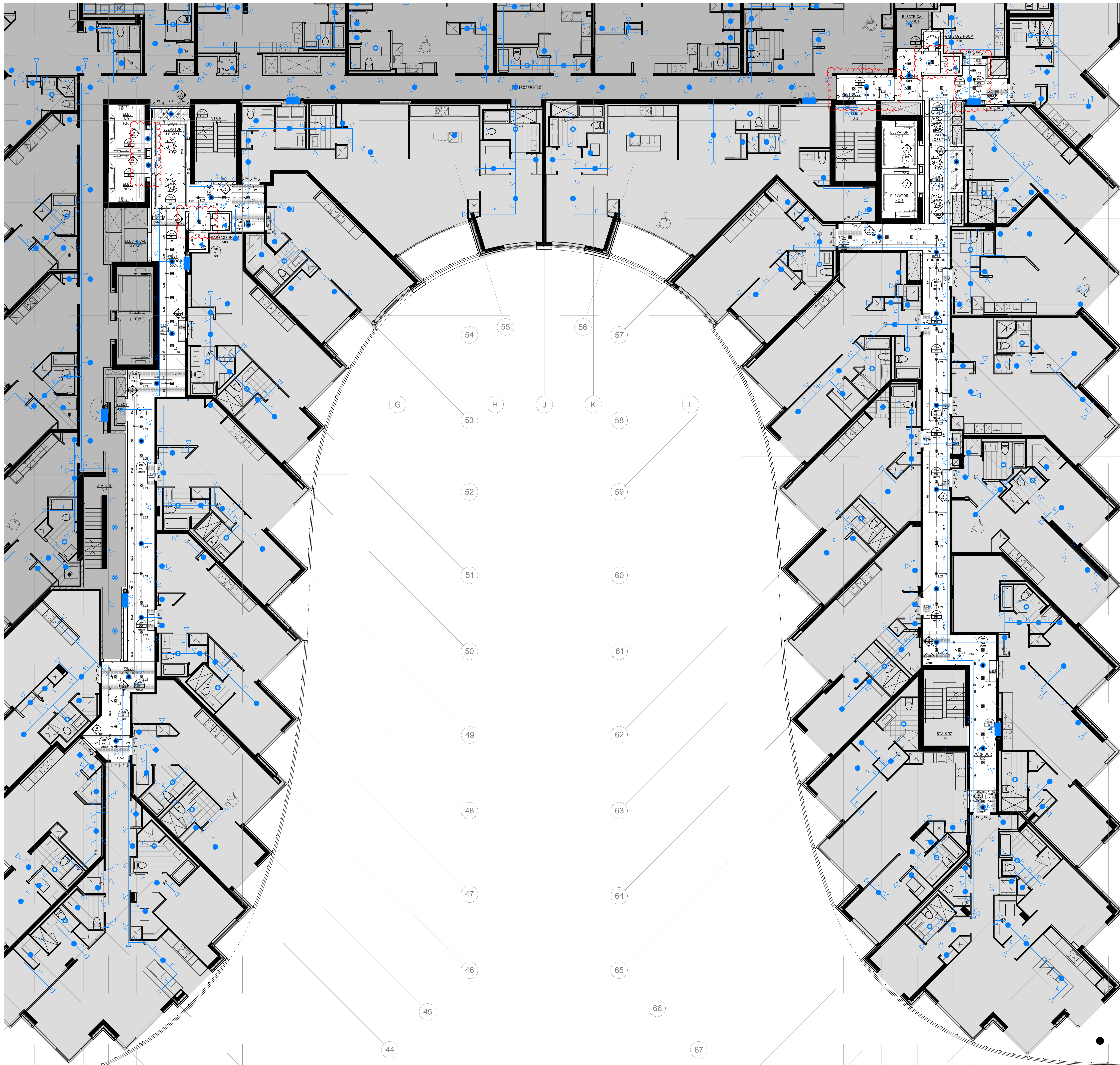
1 REFLECTED CEILING PLAN (R1.1) SCALE: 1:7.5
