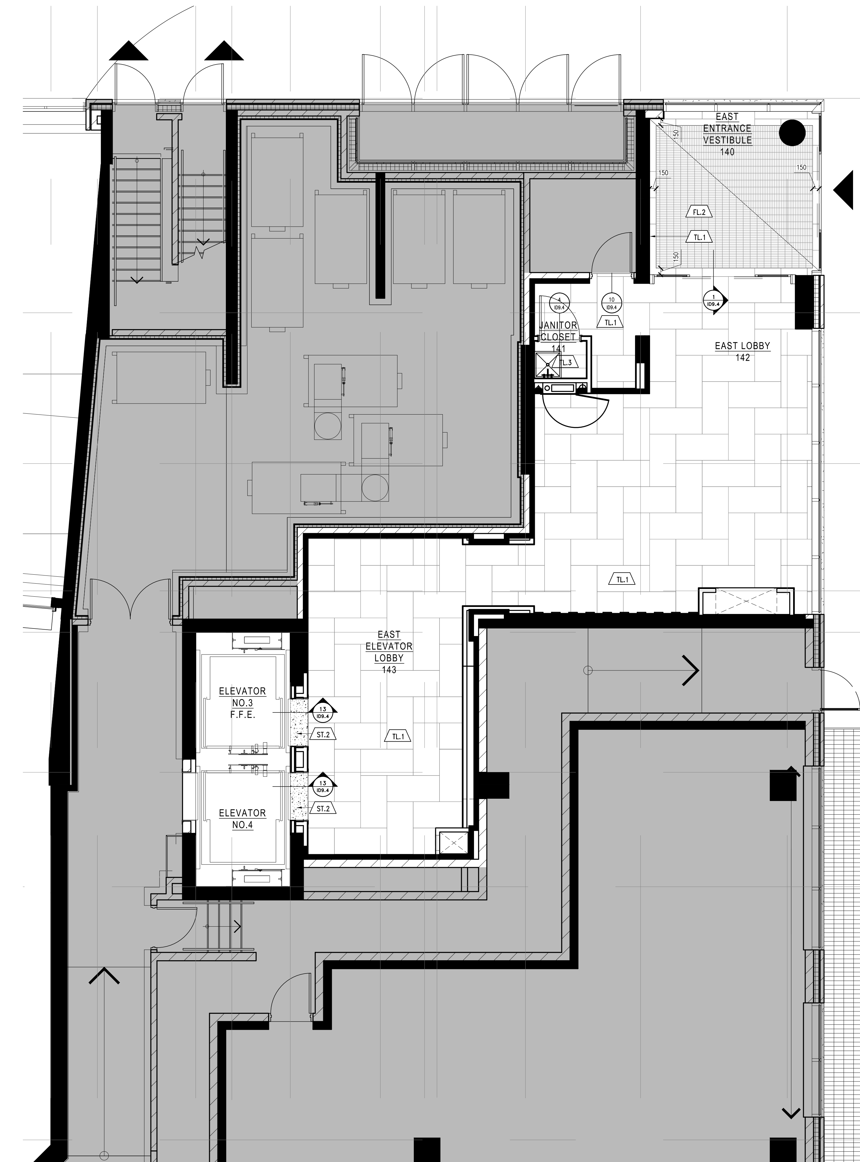
2 FLOOR FINISH PLAN SCALE: 1:50
