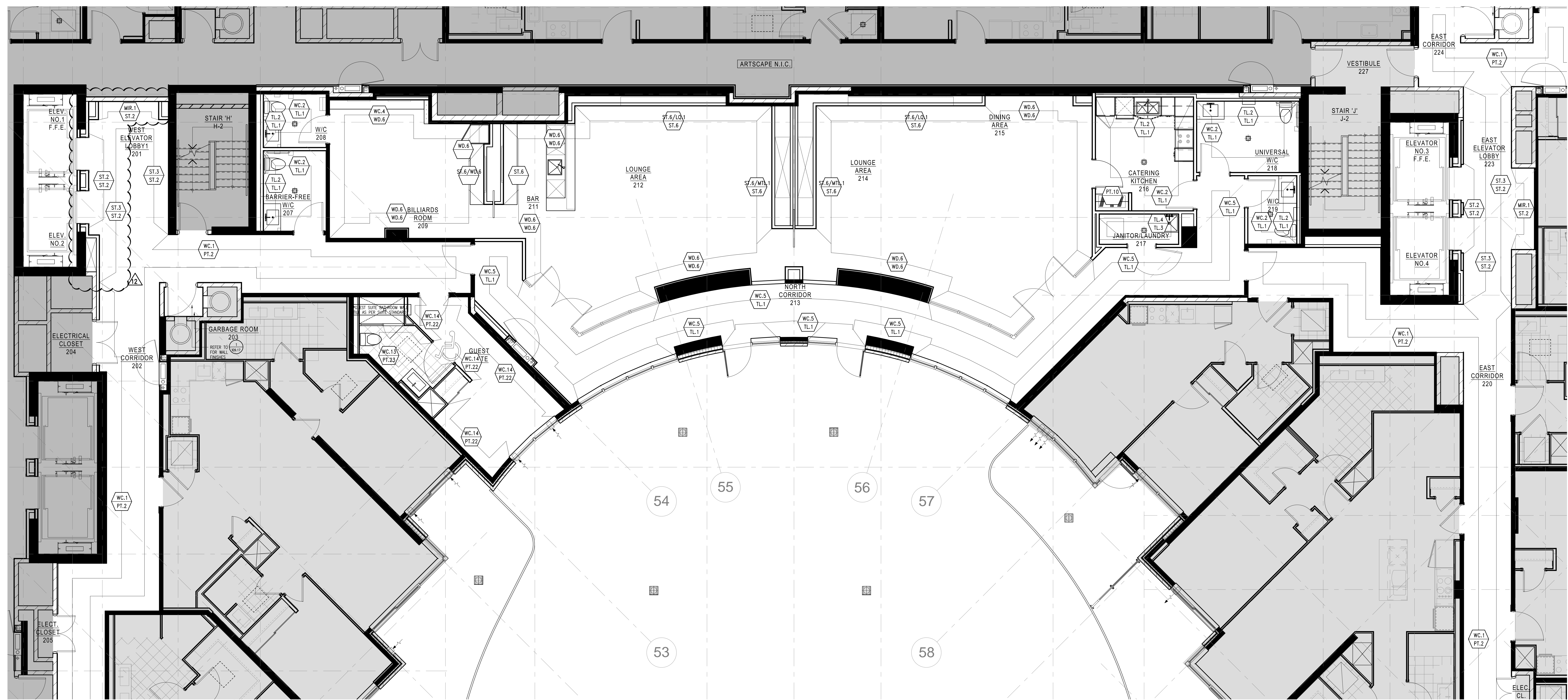
1 WALL FINISH PLAN SCALE 1:50
