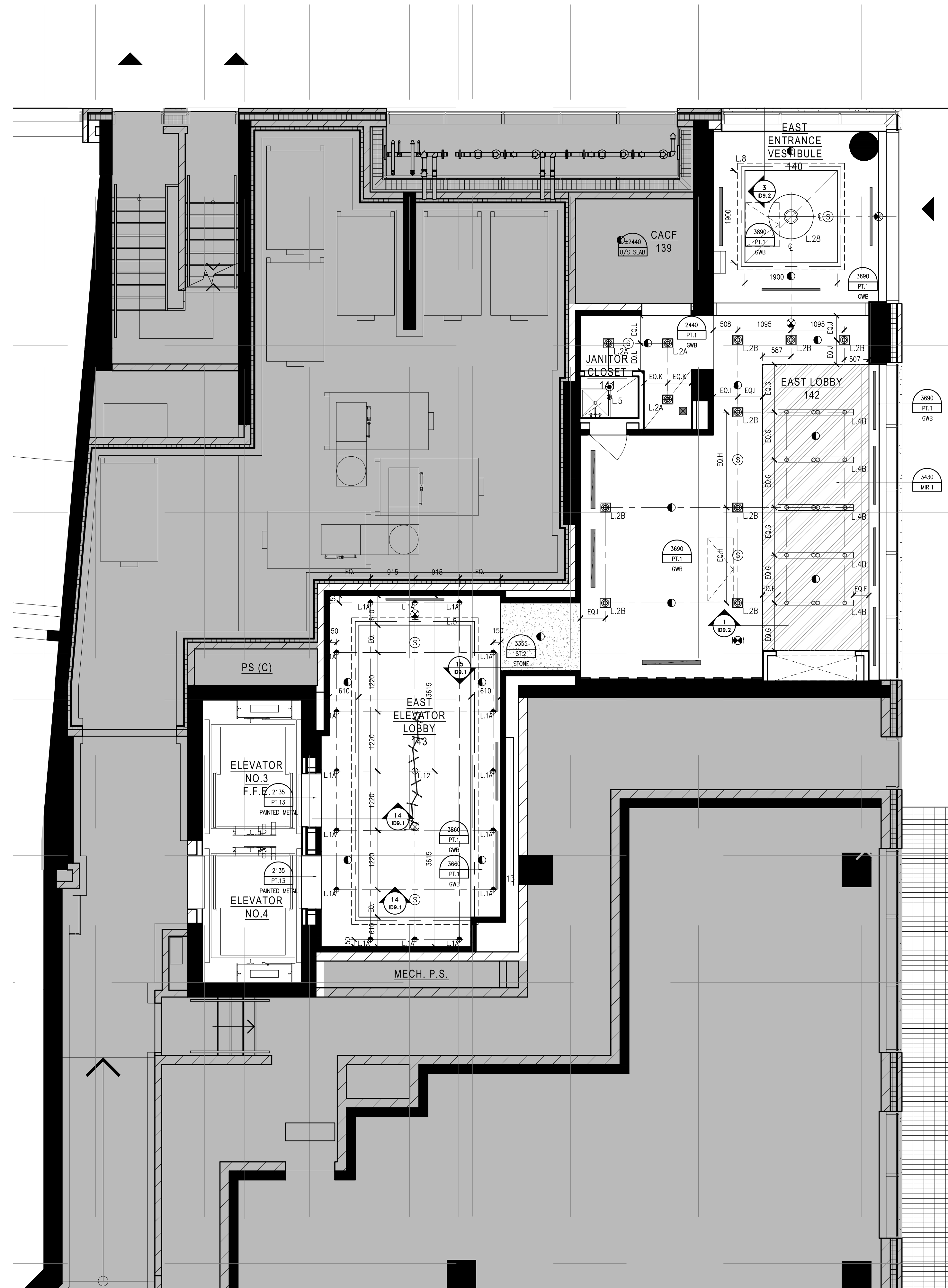
2 REFLECTED CEILING PLAN ID3.6 SCALE 1:50
