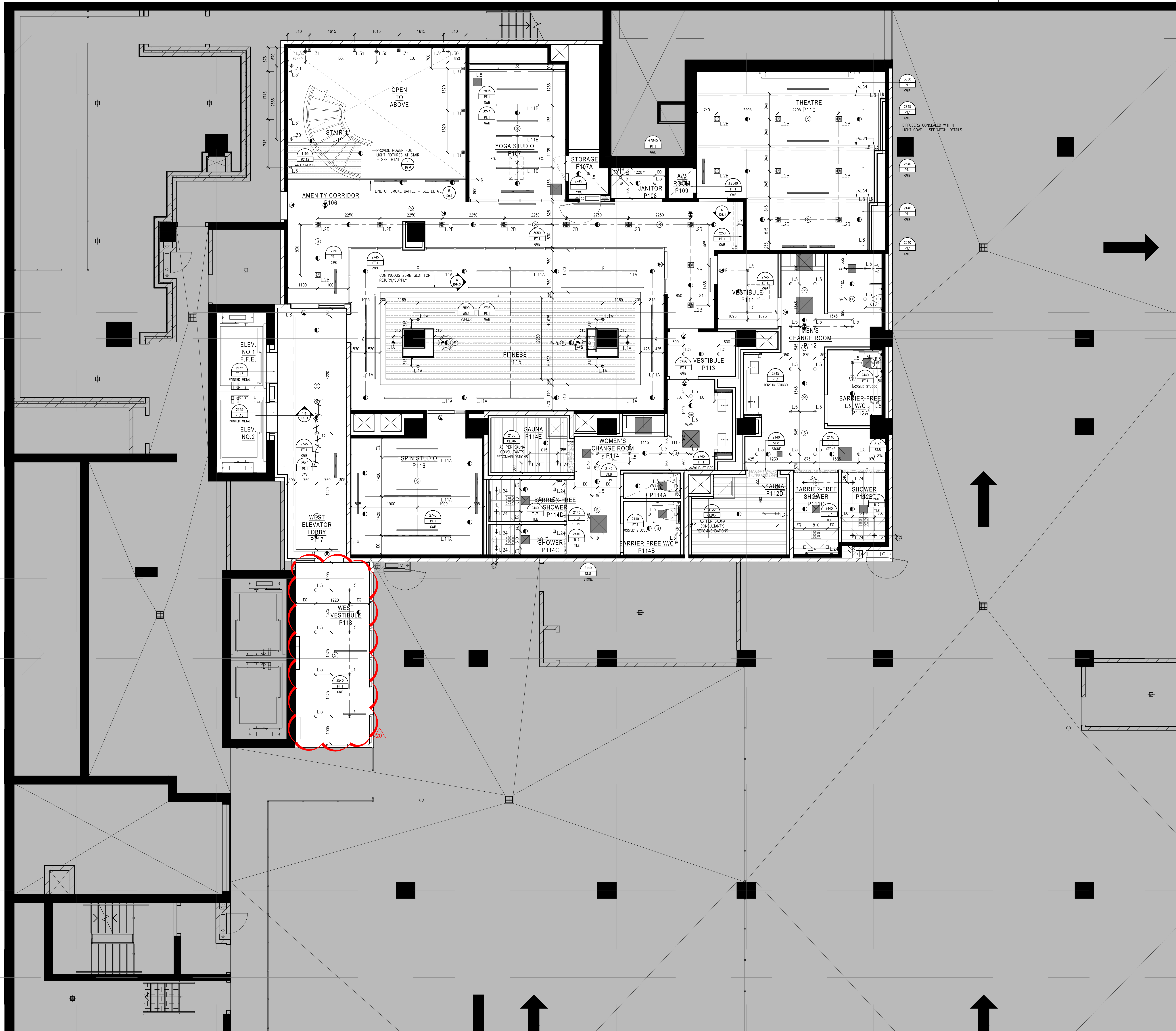
1 REFLECTED CEILING PLAN SCALE: 1:50
