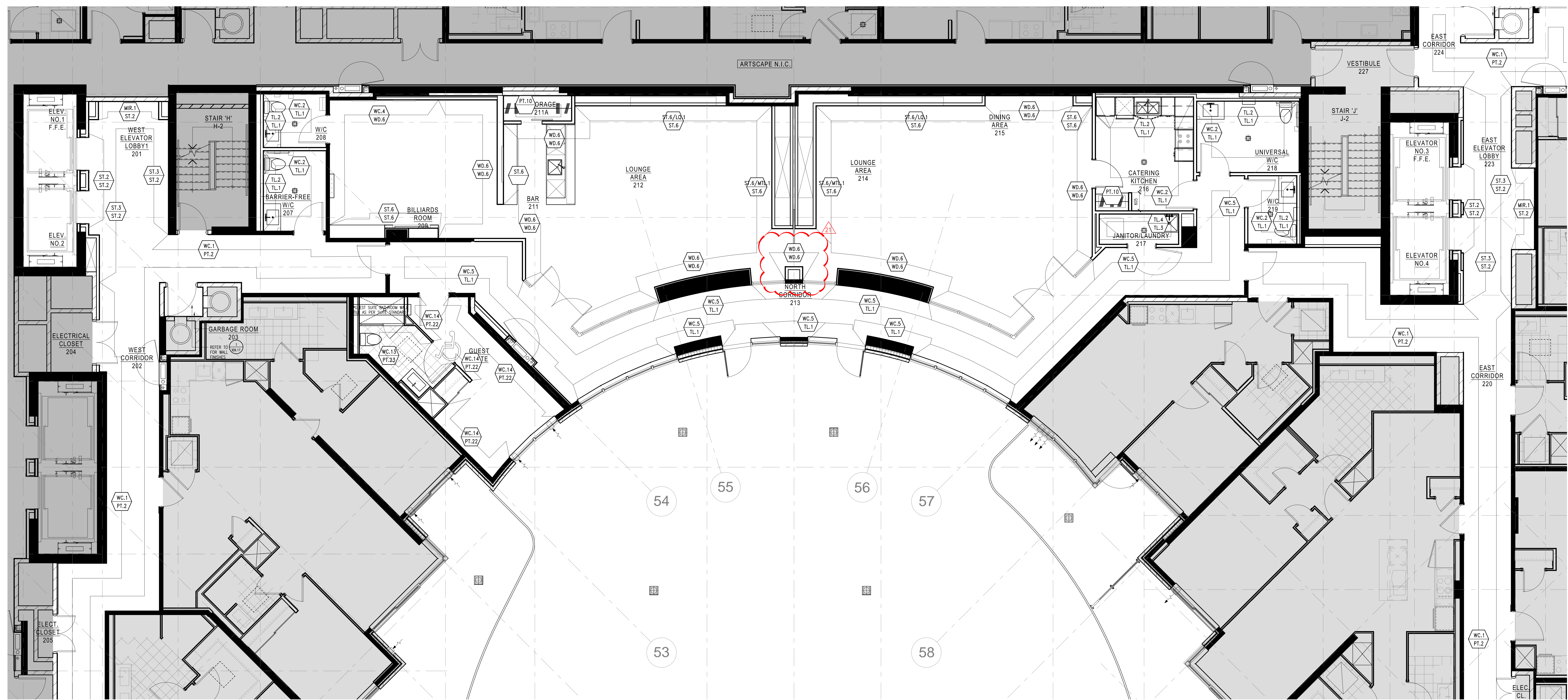
1 WALL FINISH PLAN 06.84 SCALE 1:50
