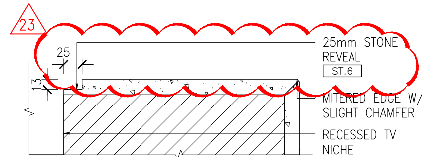
3 DETAIL — FEATURE WALL D2.01.1 SCALE 1:5
