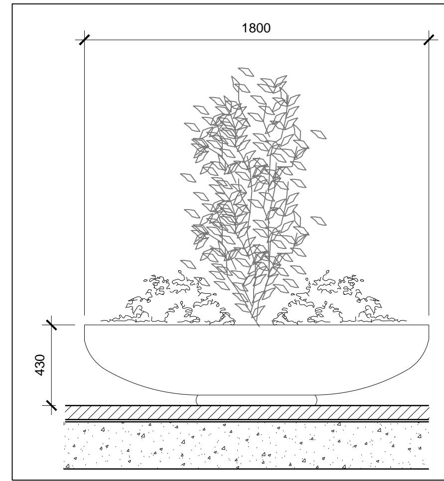
2 CONTEMPRA PLANTER BY BARKMAN SCALE: 1 : 20
